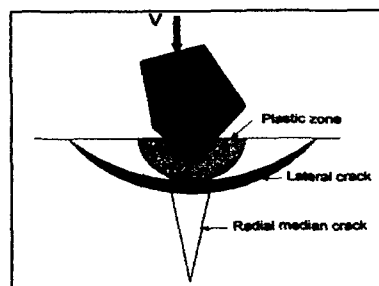
Fig. 2 Erosion mechanism by a single particle impact
