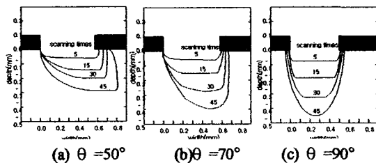
Fig. 14 Experimental profiles plotted schematically (d=7cm, pattern width=0.5mm)
