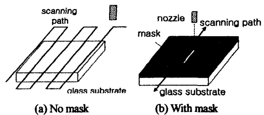
Fig. 5 Nozzle scanning path.
