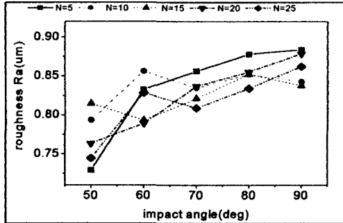
Fig. 8 Effect of the impact angle on the surface roughness for different scanning times (d=7cm)
