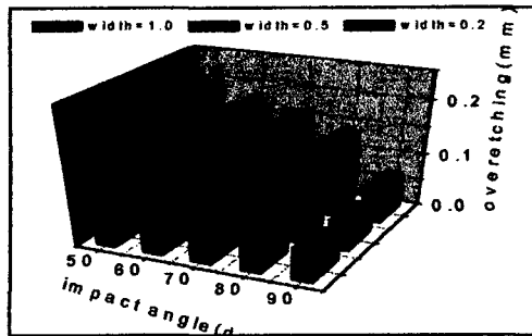
Fig. 13 Total overetching (d=7cm, N=30)
