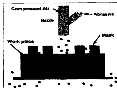
Fig. 1 A schematic principle of powder blasting.
