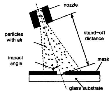
Fig. 4 A schematic view of experimental set-up
