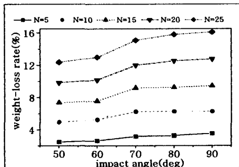
Fig.6 Effect of the impact angle on the weight-loss rate for different scanning times (d=7cm)
