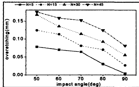
Fig. 12 Total overetching(d=7cm, pattern width=0.5mm)
