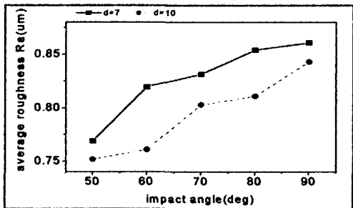
Fig.9 Averaged surface roughness as a function of the impact angle. (d=7cm)
