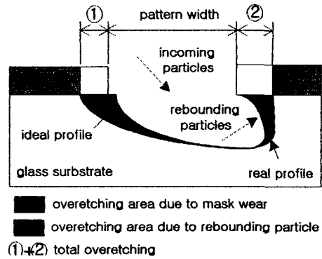
Fig. 11 Schematic wall profile and overetching
