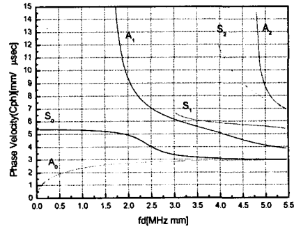
Fig. 2 Dispersion curve for steel(phase velocity)
