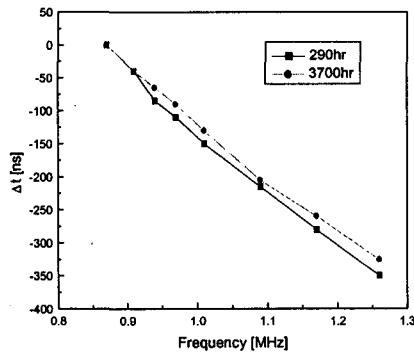
Fig. 13 Time delay of A_1 mode with respect to frequency sweeping over the range of (0.87MHz ~ 1.26MHz)
