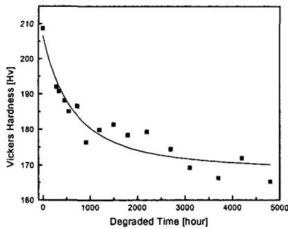
Fig. 6 Change of Vickers hardness with degraded time
