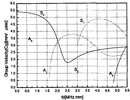
Fig. 3 Dispersion curve for steel(group velocity)
