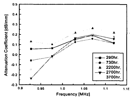
Fig. 8 Attenuation coefficient of A_1 mode measured by Lamb wave
