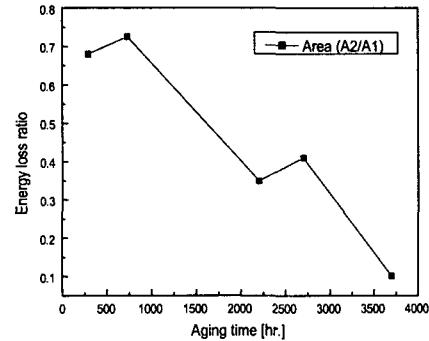
Fig. 11 The variation of A_1 energy loss ratio at f=1\text{MHz} with respect to aging time
