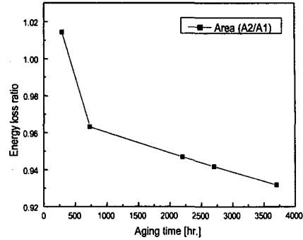
Fig. 10 The variation of S_0 energy loss ratio at f=1\text{MHz} with respect to aging time
