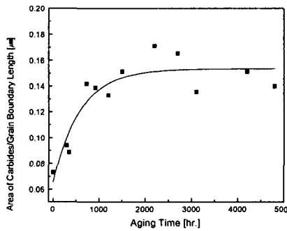
Fig. 7 Change of area on grain boundary carbides per unit grain boundary length
