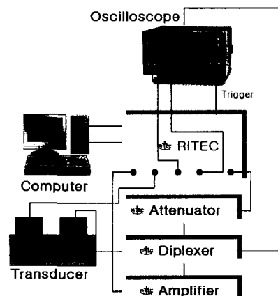
Fig. 4 Schematic diagram of the experimental set-up
