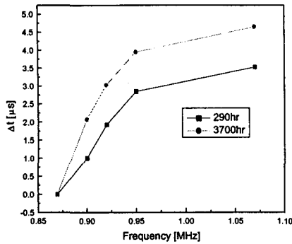
Fig. 12 Time delay of S_0 mode with respect to frequency sweeping over the range of (0.87MHz ~ 1.07MHz)
