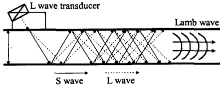
Fig. 1 Oblique incidence method for the generation of Lamb wave
