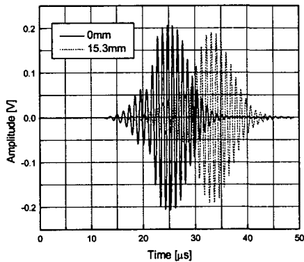
Fig. 9 RF-signal of Lamb wave over the distance (0mm ~ 15.3mm)
