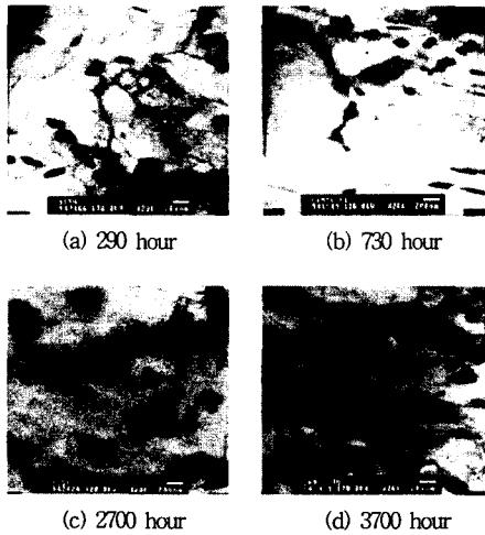
Fig. 5 TEM micrographs showing morphology of carbide
