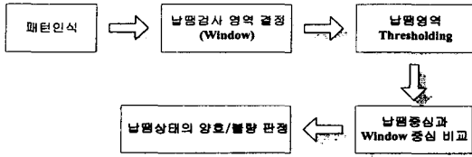
Fig. 4 Flowchart of solder test.
