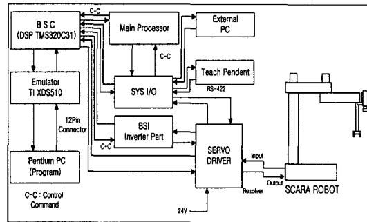
Fig. 6. The block diagram of control system.
