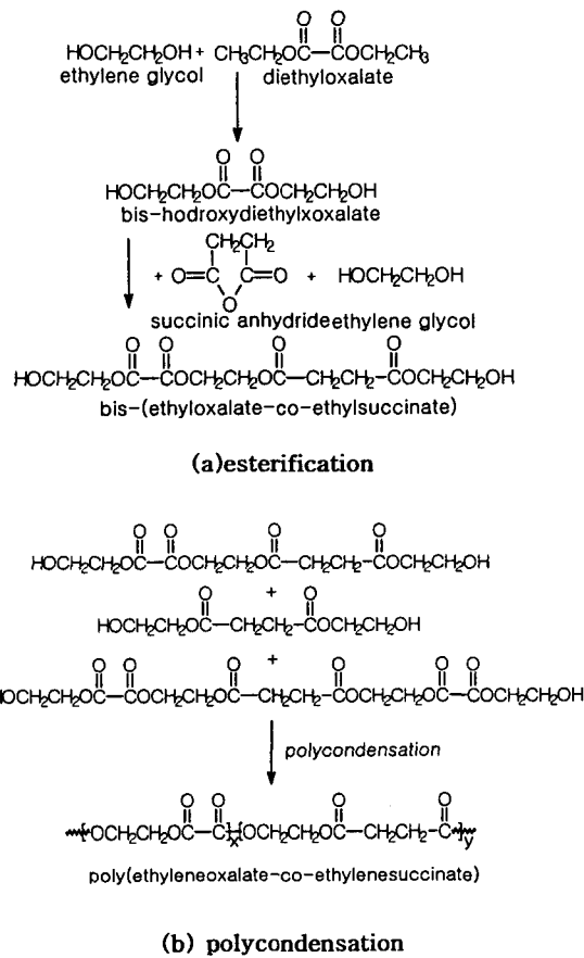
Fig. 1 Reaction scheme of poly(ethylene succinate-co-ethylene oxalate)
