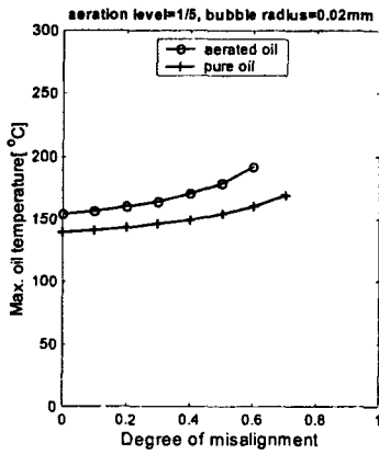
Fig. 19 Maximum oil temperature vs. degree of misalignment, aeration level=1/5, bubble radius=0.02mm
