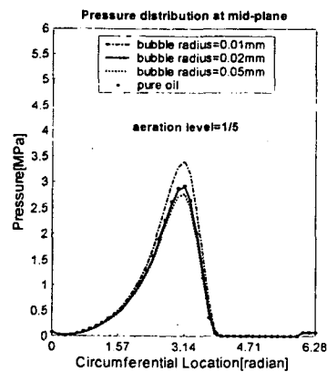
Fig. 9 Pressure distribution at bearing mid-plane, r_{in}/d_{in}=1/5
