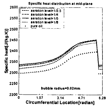
Fig. 8 Specific heat distribution at bearing mid-plane, r_{in}=0.02mm
