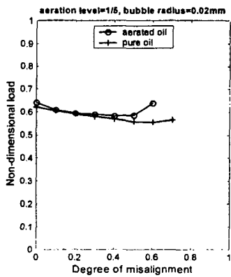
Fig. 20 Non-dimensional load vs. degree of misalignment, aeration level=1/5, bubble radius=0.02mm
