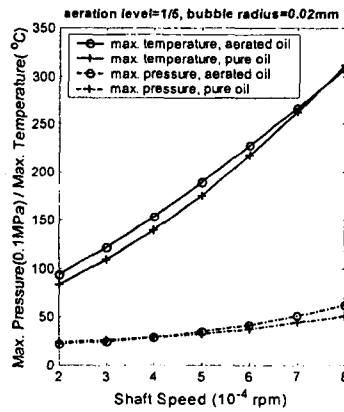
Fig. 23 Maximum pressure and temperature vs. shaft speed for an aligned bearing
