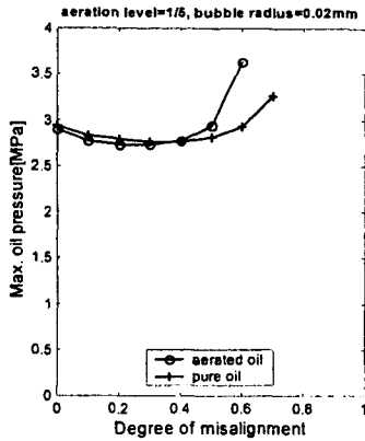
Fig. 18 Maximum oil pressure vs. degree of misalignment, aeration level=1/5, bubble radius=0.02mm
