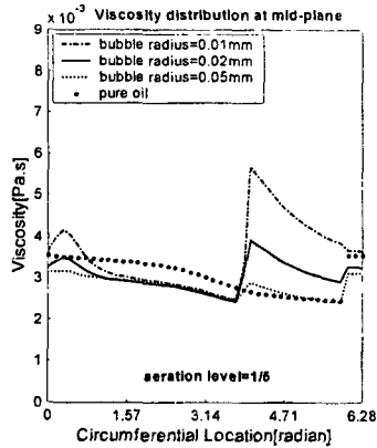
Fig. 10 Viscosity distribution at bearing mid-plane, r_{in}/d_{in}=1/5
