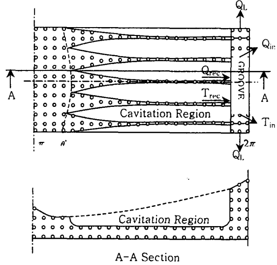
Fig. 2 Diagram of lubricant flow, with Q_i the inlet oil flow rate, Q_m the re-circulating flow rate and Q_s the side oil flow rate going through groove land. \theta^* is the angle of the beginning of the cavitation region.
