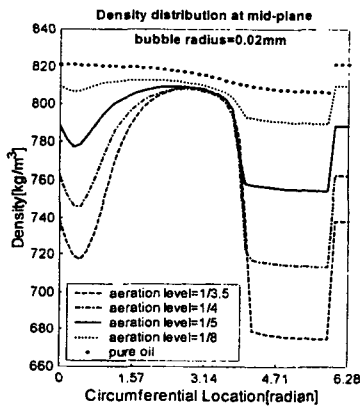
Fig. 7 Density distribution at bearing mid-plane, r_{in}=0.02mm
