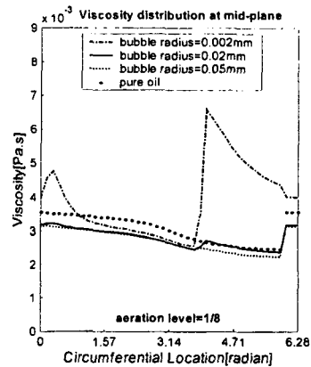
Fig. 13 Viscosity distribution at bearing mid-plane, r_{in}/d_{in}=1/8
