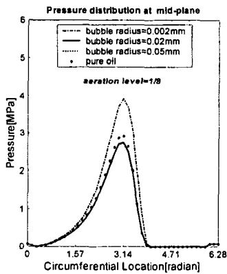
Fig. 11 Pressure distribution at bearing mid-plane, r_{in}/d_{in}=1/8
