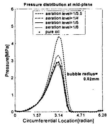
Fig. 3 Pressure distribution at bearing mid-plane, r_{in}=0.02mm
