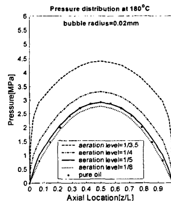
Fig. 4 Pressure distribution in axial direction at 180°, r_{in}=0.02mm
