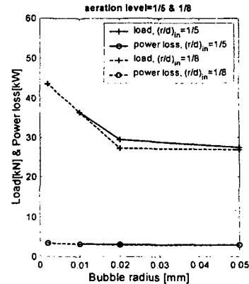
Fig. 17 Bearing load and power loss vs. bubble radius, r_{in}/d_{in}=and 1/5 and 1/8
