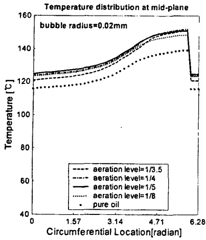
Fig. 5 Temperature distribution at bearing mid-plane, r_{in}=0.02mm
