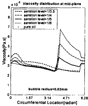
Fig. 6 Viscosity distribution at bearing mid-plane, r_{in}=0.02mm
