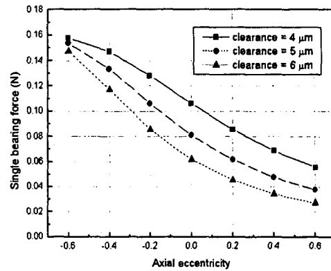
Fig. 8 Single bearing force vs. axial eccentricity of thrust bearing (with four capillaries, capillary radius= 30\ \mu\text{m} , supply pressure= 0.4\ \text{MPa} )
