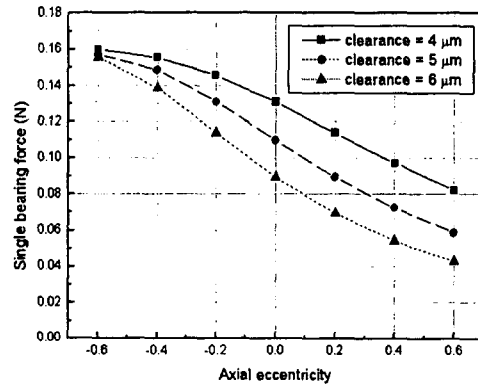
Fig. 9 Single bearing force vs. axial eccentricity of thrust bearing (with four capillaries, capillary radius= 50\ \mu\text{m} , supply pressure= 0.4\ \text{MPa} )
