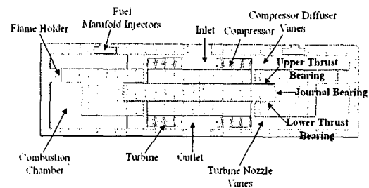
Fig. 2 Cut-away view of Micro Gas Turbine
