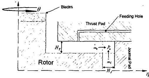
Fig. 3 Schematics of coupled control volume
