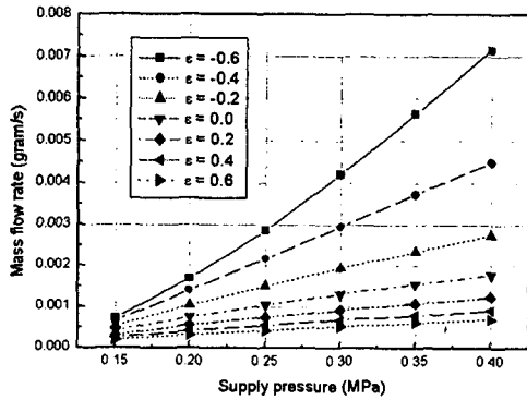
Fig. 5 Mass flow rate vs. supply pressure of single thrust bearing (with four capillaries, capillary radius=50 \mu\text{m} , clearance=10 \mu\text{m} )
