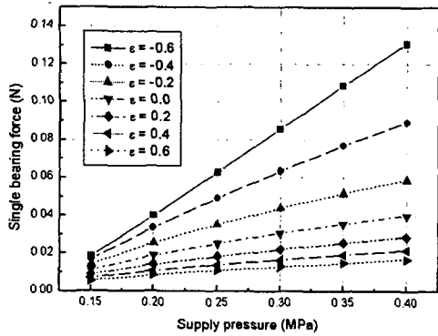
Fig. 4 Bearing force vs. supply pressure of single thrust bearing (with four capillaries, capillary radius=50 \mu\text{m} , clearance=10 \mu\text{m} )
