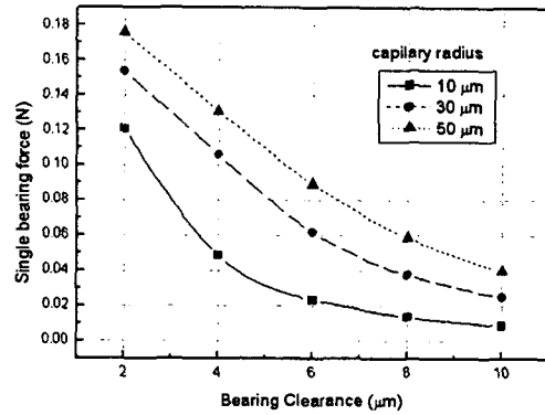
Fig. 6 Single bearing force vs. bearing gap of thrust bearing (with four capillaries, supply pressure=0.4 MPa, axial eccentricity ratio=0)
