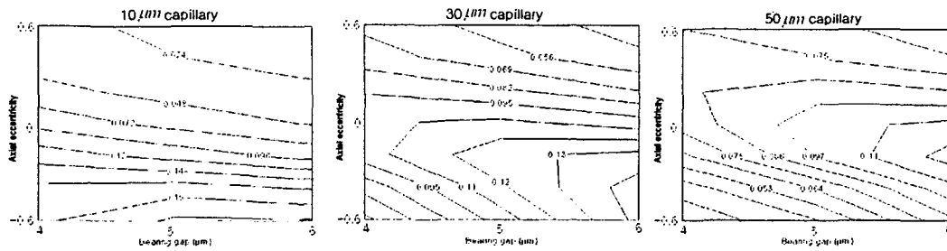
Fig. 10 Slope contour of single bearing force vs. axial eccentricity curves (with four capillaries, supply pressure=0.4 MPa)
