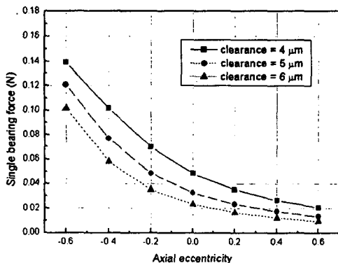
Fig. 7 Single bearing force vs. axial eccentricity of thrust bearing (with four capillaries, capillary radius= 10\ \mu\text{m} , supply pressure= 0.4\ \text{MPa} )
