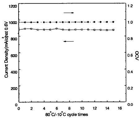
Fig. 3. Performance of single cell at 80°C for 80°C/-10°C cycle times. non-humidified gas purging for 30 minutes.
