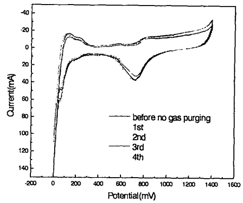
Fig. 6. Cyclic voltammograms at 80°C for 80°C/-10°C cycle times. no gas purging
