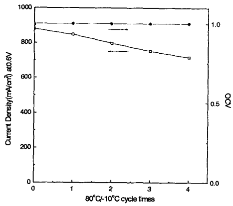
Fig. 5. Performance of single cell at 80°C for 80°C/-10°C cycle times. no gas purging
