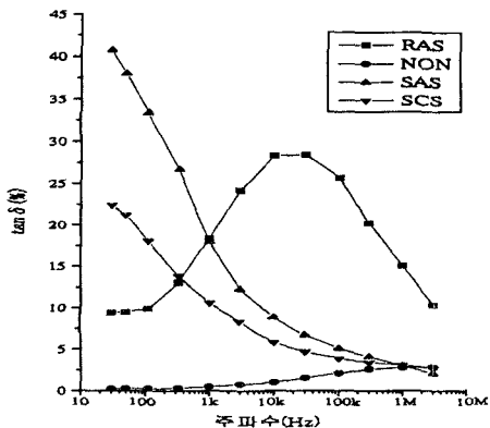
Fig. 5 The frequency properties of \text{Tan } \delta vs. filler shapes(25°C)
