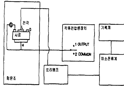
Fig. 3 Measured device circuit charge and discharge current
