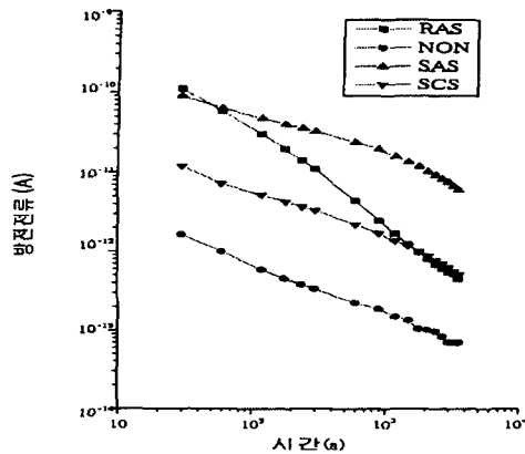
Fig. 7 The properties of discharge current due to time vs. filler shapes (25°C Vb=-500V)
