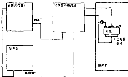
Fig. 2 Measured device circuit dielectric loss
