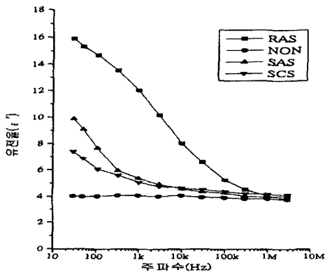
Fig. 4 The frequency properties of \epsilon' vs. filler shapes(25°C)
