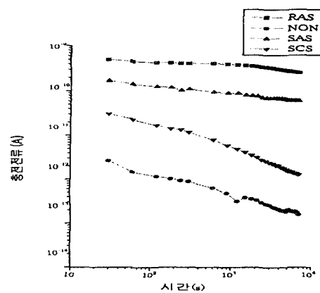
Fig. 6 The properties of charge current due to time vs. filler shapes (25°C V_b = -500V )
