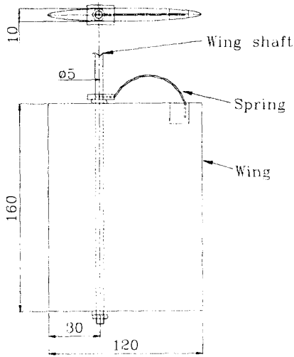
Fig. 7 Structure of wing (unit : mm)
