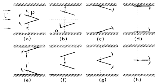
Fig. 2 A model of propulsion mechanism (Model I)
