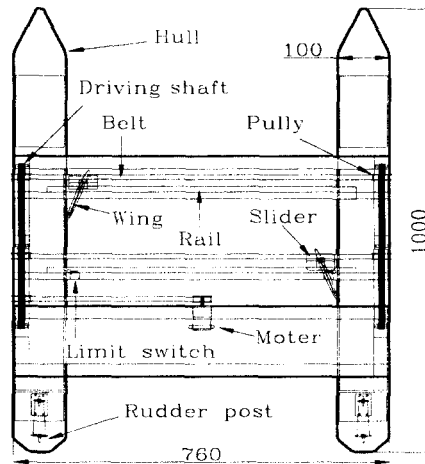
Fig. 5 Schematic diagram of model ship (unit :mm)
