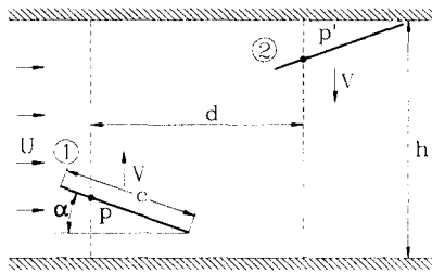
Fig. 4 A model of propulsion mechanism (Model III)
