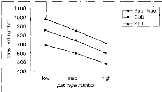
Fig. 3 (a) The number of tardy parts according to the number of part types
