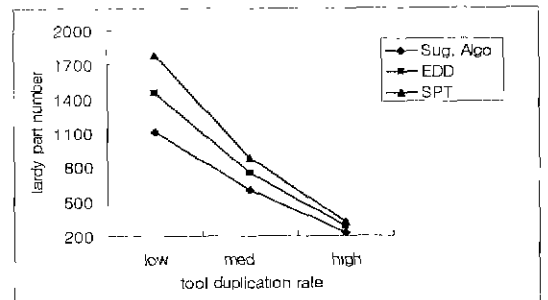
Fig. 2 (a) The number of tardy parts by varying tool duplication rate
