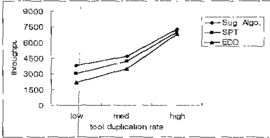
Fig. 2 (b) The throughput by varying tool duplication rate
