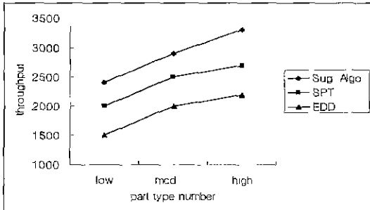
Fig. 3 (b) The throughput according to the number of part types
