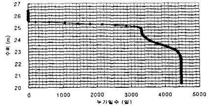
Fig. 6 Cumulative day-Suction water level of Paldang 1st pump station(1984~1998년)
