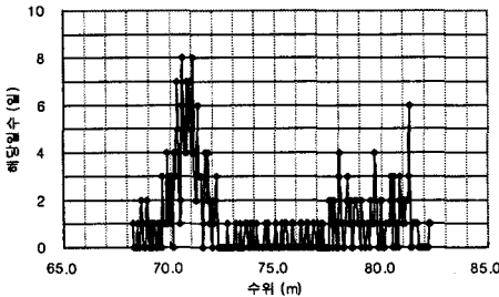
Fig. 9 Discharge water level of Paldang 1st pump station(998년)
