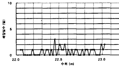
Fig. 7 Discharge water level of Jayang pump station(1998년)
