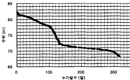
Fig. 10 Cumulative day-discharge water level of Pal dang 1st pump station(1998년)
