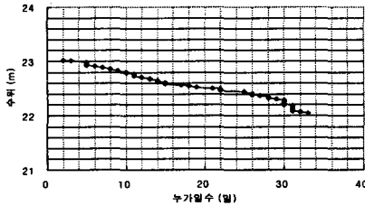
Fig. 8 Cumulative day-discharge water level of Jayang pump station(1998년)
