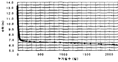
Fig. 4 Cumulative day-Suction water level of Jayang pump station(1993~1998년)
