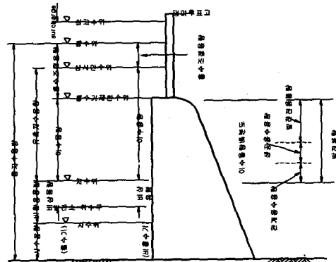
Fig. 2 Capacity distribution and water level of multipurpose dam
