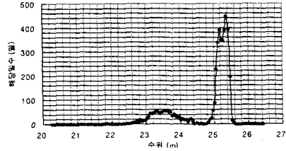
Fig. 5 Suction water level of Paldang 1st pump station(1984~1998년)
