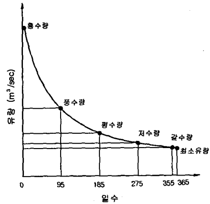
Fig. 1 Flow duration curve of river
