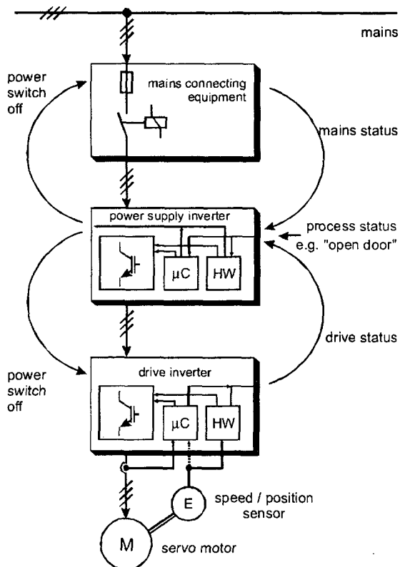
Fig. 8 Redundant structure for safe operation
