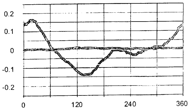
Fig. 3 Comparison of position accuracies when using magnetic or optical sensors in servo drives ([12])
