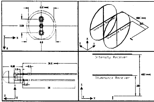
Fig. 3.1 Structure of the standard source.
