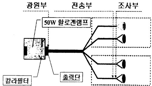
Fig. 2.1 Structure of an optical fiber lighting systems.
