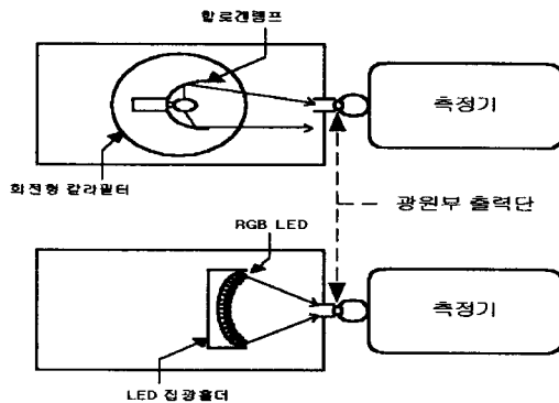
Fig. 4.1 Measurement method of the data.
