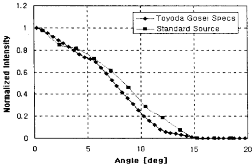
Fig. 3.2 Normalized intensity of Toyoda Gosei Co., LTD. LED specs vs. standard source.
