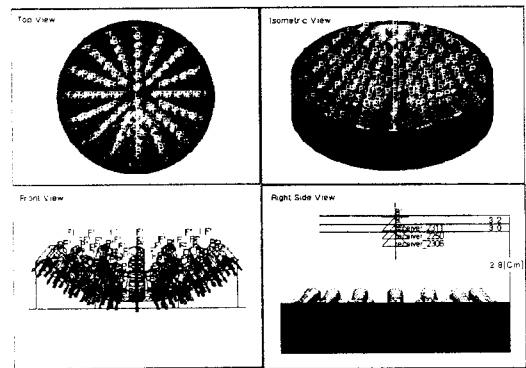
Fig. 3.6 Structure of a light collecting holder.
