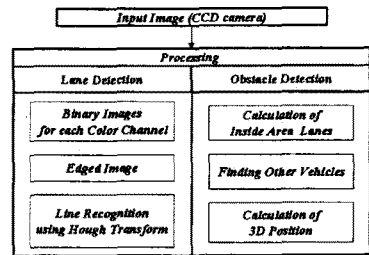
Fig. 1 Block diagram of processes
