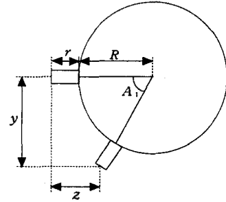
Fig.4. Kinematic analysis of the bottom of the cylinder
