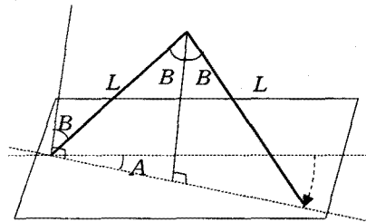
Fig.5 Kinematic analysis of the plane
