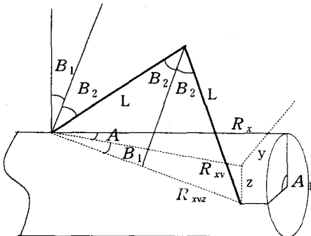
Fig.3. Kinematic analysis of the cylinder surface
