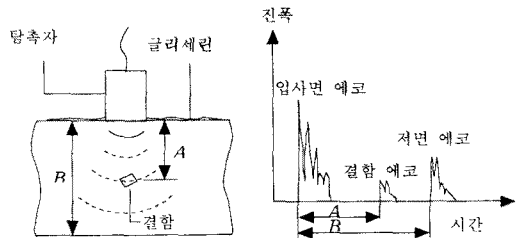
Fig.1. A fundamental theory of ultrasonic inspection
