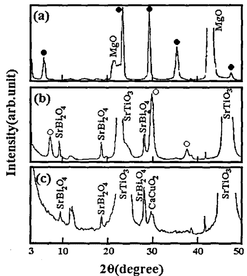
Fig. 1. XRD patterns of (a) co-deposited and (b), (c) layer-by-layer deposited thin film. Marks of \bullet , \circ , \triangle and \square indicate Bi2212, Bi2201, SrBi 2 O 4 and, CaCuO 2 respectively.
