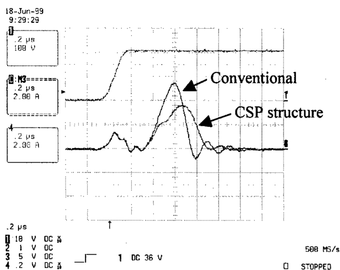
Fig. 2. The discharge current wave form measured during sustain period.
