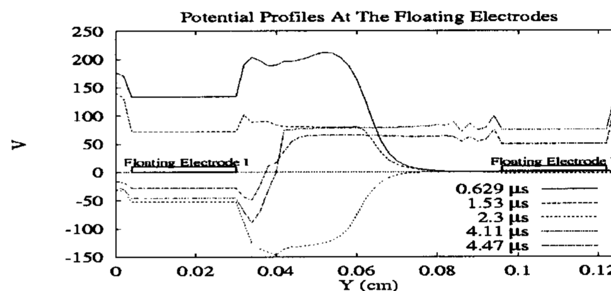
Fig. 4. Simulation result of the electric potential line in the new structure
