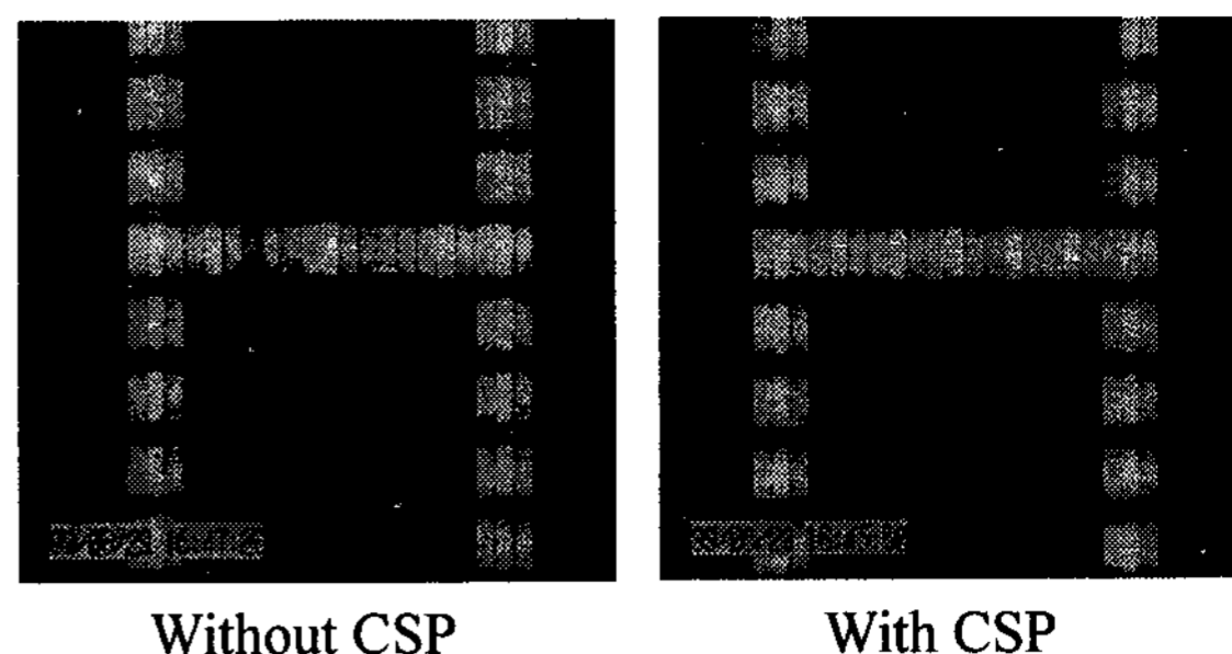
Fig. 3. Cross talk without CSP and with CSP
