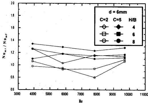
Fig. 7 Average Nusselt number ratio for Reynolds number on various H/B
