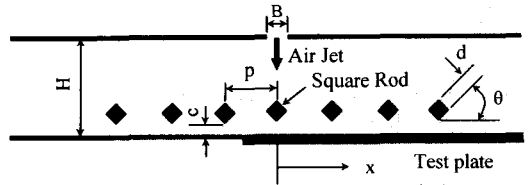
Fig. 2 Cross-sectional view of test section and coordinate system
