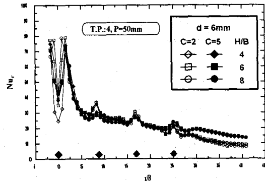
(b) Re = 9700
