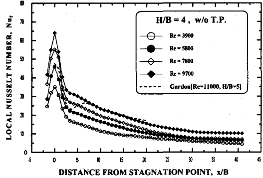
(a) H/B = 4
