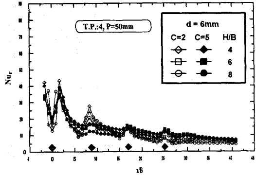
(a) Re = 3900
