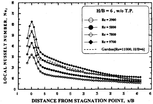
(b) H/B = 6
