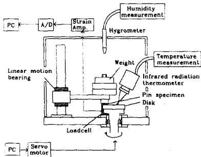
Fig. 2-1 Schematic of test apparatus
