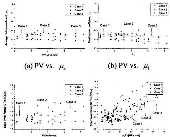
Fig.3-14 Comparison of the results of Case 1, Case 2 and Case 3
