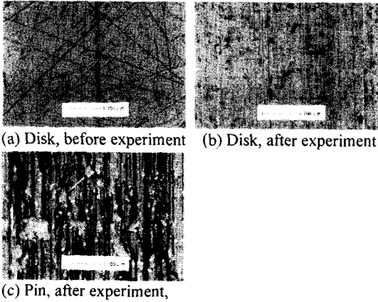
Fig.3-7 Pin and disk surfaces when the severe abrasive occurred on the disk ( P = 5.53 \text{ MPa} , V = 0.5 \text{ m/s} )
