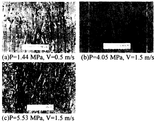
Fig.3-11 Pin surfaces after experiment in case of Case 3
