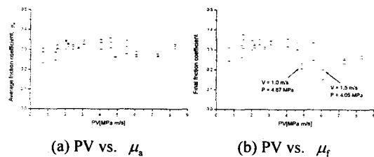
Fig.3-12 PV vs friction coefficient in case of Case 3
