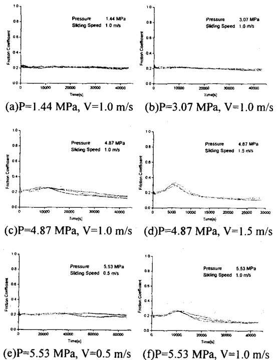
Fig.3-1 Variation of friction coefficient with time in case of Case 1( R_{\text{max}} ; 1.5\mu\text{m} \sim 3.5\mu\text{m} , HRC; 31~34)
