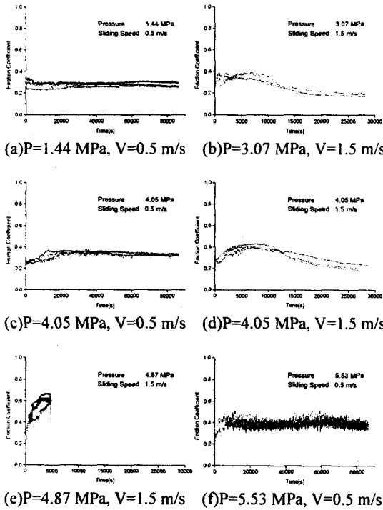
Fig.3-5 Variation of friction coefficient with time in case of Case 2 ( R_{max} ; 0.3 \mu m \sim 0.8 \mu m , HRC; 32~34)
