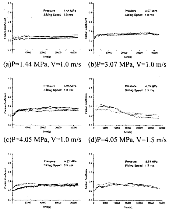
Fig.3-10 Variation of friction coefficient with time in case of Case 3 ( R_{max} ; 1.2 \mu\text{m} \sim 3.0 \mu\text{m} , HRC ; 61~63)
