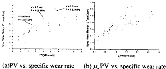
Fig.3-13 Specific wear rate in case of Case 3
