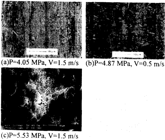
Fig.3-2 Pin surfaces after experiment in case of Case 1
