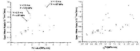
Fig.3-9 Specific wear rate in case of Case 2
