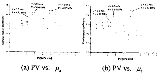
Fig.3-8 PV vs. friction coefficient in case of Case 2
