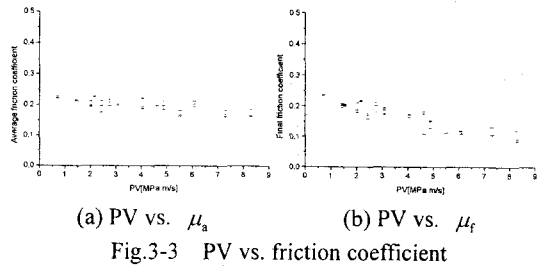
Fig.3-3 PV vs. friction coefficient
