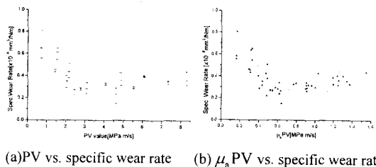
Fig.3-4 Specific wear rate in case of Case 1
