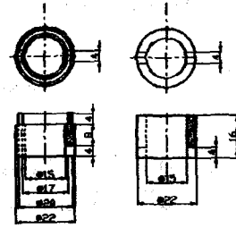
Fig. 2 Shape and dimensions of specimens
