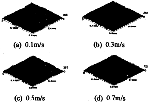
Fig. 8 Simulation of frictional surface by image processing ; applied load : 10kg, sliding distance : 1.0km
