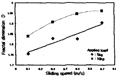
Fig. 9 Fractal dimension of frictional surface for sliding speed; sliding distance : 1.0km
