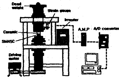
Fig. 1 Schematic diagram of experimental unit
