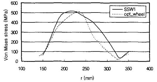
Fig. 10 Comparison of Von Mises stress distribution in wheel plate radius on FFS due to the thermal load
