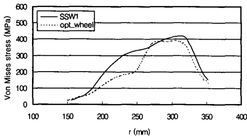
Fig. 13 Comparison of Von Mises stress distribution in wheel plate radius on BFS due to the combined load
