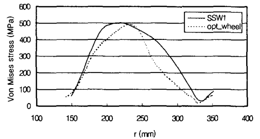
Fig. 12 Comparison of Von Mises stress distribution in wheel plate radius on FFS due to the combined load
