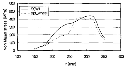
Fig. 11 Comparison of Von Mises stress distribution in wheel plate radius on BFS due to the thermal load
