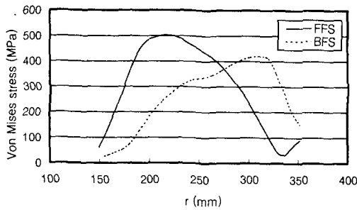
Fig. 4 Von Mises stress distribution in wheel plate radius due to the combined load
