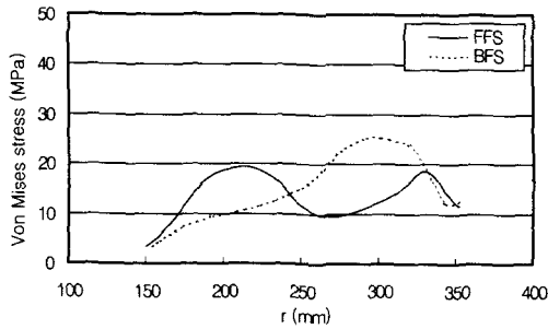
Fig. 2 Von Mises stress distribution in wheel plate radius due to the mechanical load
