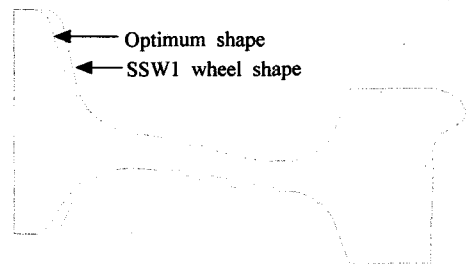
Fig. 7 Comparison optimum shape with SSW1 wheel shape
