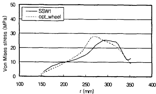
Fig. 9 Comparison of Von Mises stress distribution in wheel plate radius on BFS due to the mechanical load
