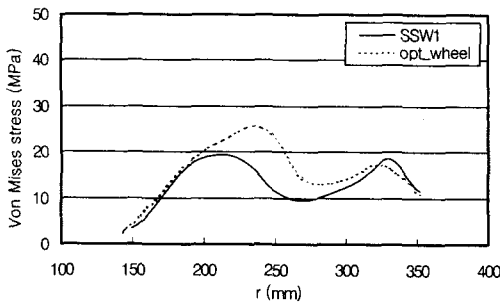
Fig. 8 Comparison of Von Mises stress distribution in wheel plate radius on FFS due to the mechanical load
