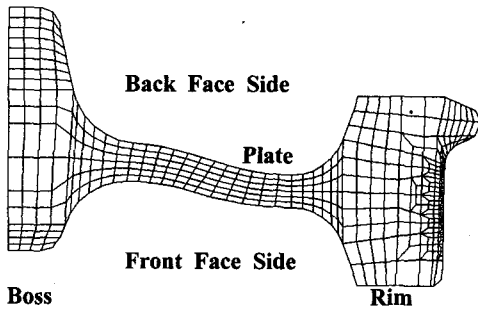
Fig. 1 Section of 3-dimensional finite element model
