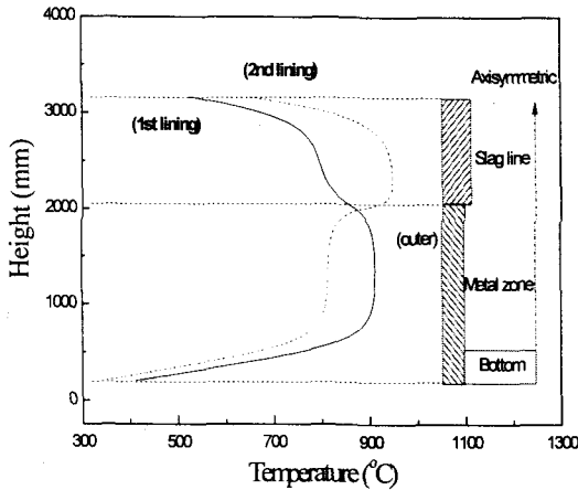
Fig. 5 Temperature distribution at back face(outer) of dolomite brick
