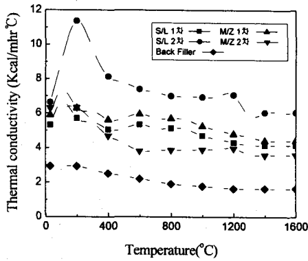
Fig. 2 Thermal conductivities of each material
