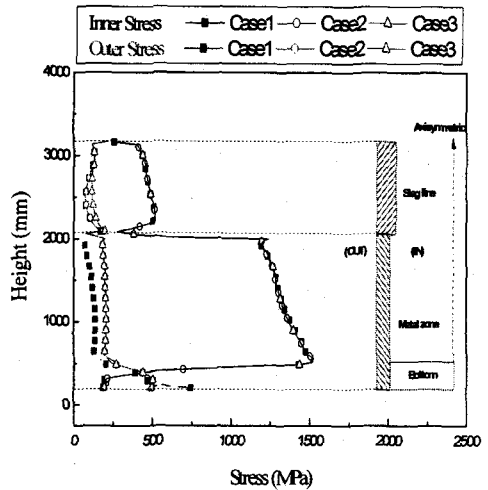
Fig. 9 Thermal Stress at hot face(inner) and back face(outer) of dolomite brick
