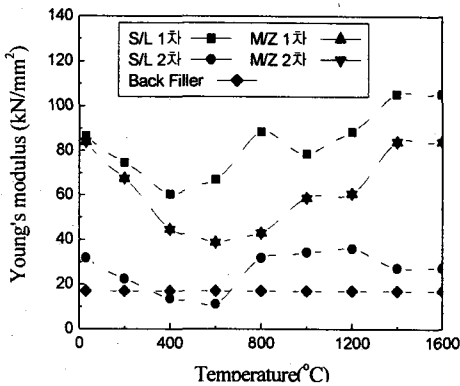
Fig. 3 Young's modulus of each material
