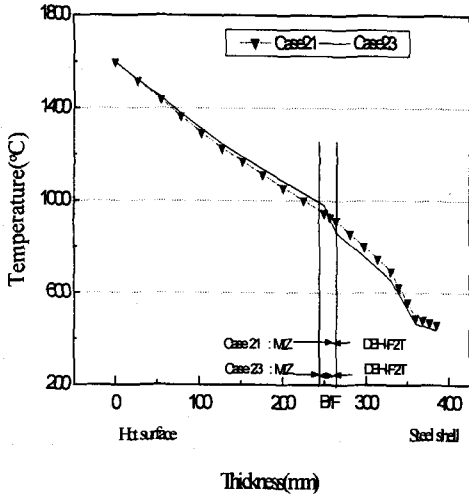
Fig. 7 Thermal distribution by construction of B/F at slag line
