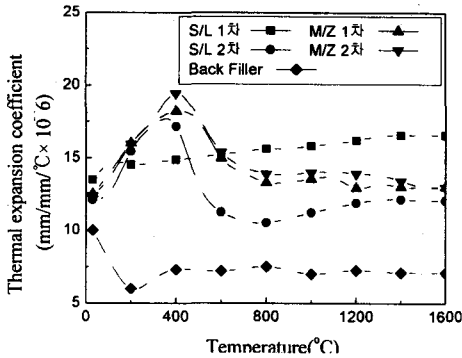
Fig. 4 Thermal expansion coefficient of each material
