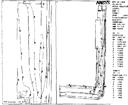
Fig. 10 Analysis of thermal stress without back filler in 2nd lining
