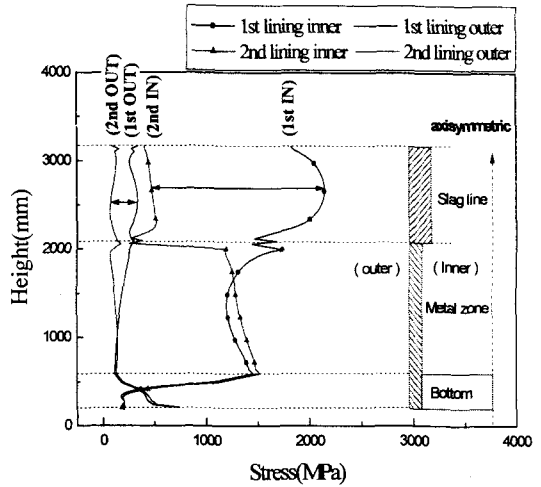
Fig. 6 Thermal Stress at hot face(inner) and back face(outer) of dolomite brick
