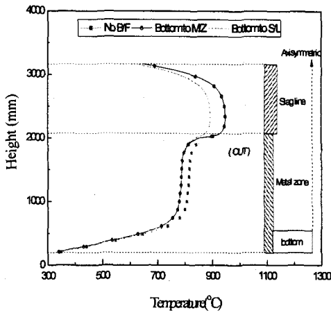
Fig. 8 Temperature distribution at back face(outer) of dolomite brick
