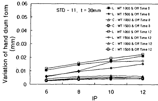
Fig. 4 The measured Hand drum form with IP between the square hole and the circle hole
