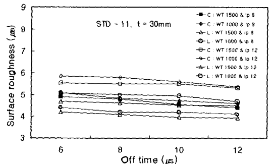
Fig. 1 The measured Surface Roughness with tension between the square hole and the circle hole
