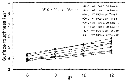
Fig. 2 The measured Surface Roughness with IP between the square hole and the circle hole
