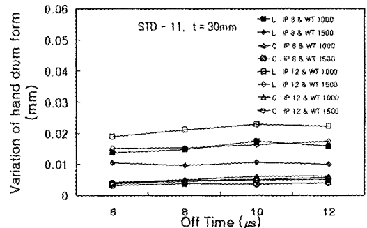
Fig. 3 The measured Hand drum form with off time between the square hole and the circle hole
