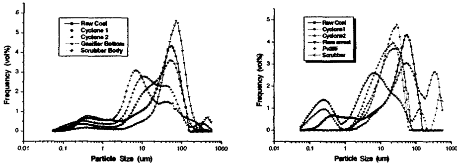
Fig. 4 Particle Size Analysis of Coal & Solid Samples
