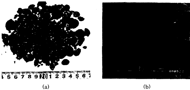
Fig. 3 Digital Photo/SEM Analysis of Adaro Coal Ash Slag (17Kg/cm 2 , 1450~1500℃, ×75)
