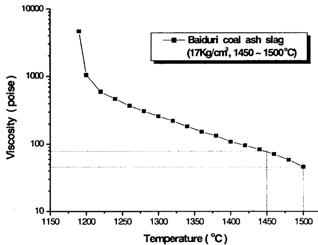
Fig. 1 Viscosity of Baiduri Coal Ash Slag
