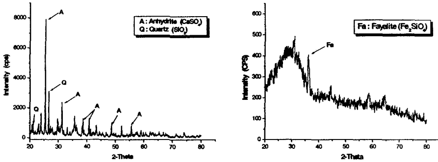
Fig. 2 XRD Analysis of Adaro Coal Ash and Slag
