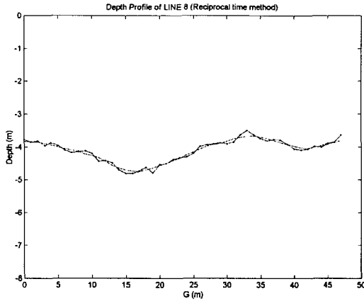
Fig. 6. Depth profile obtained with reciprocal time method
