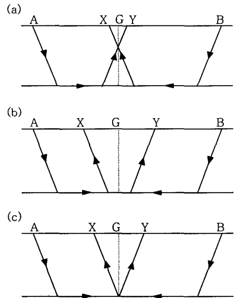
Fig. 4. Generalized Reciprocal Method
