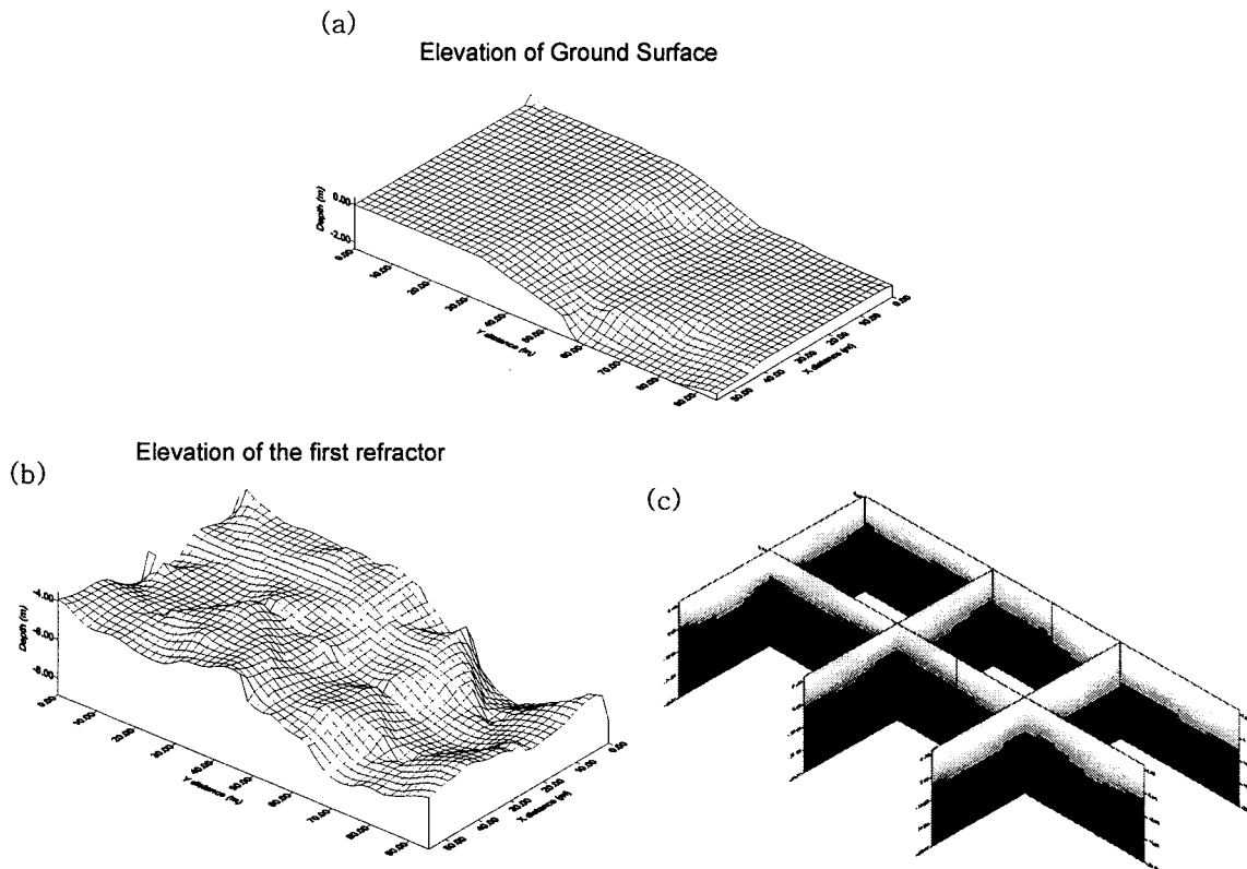
Fig. 9. Result of data processing (a) topography of the survey area, (b) the surface of the first refractor, (c) result of travel time tomography. The vertical scale of (c) is 4.4 times the vertical scale of (a) and (b)
