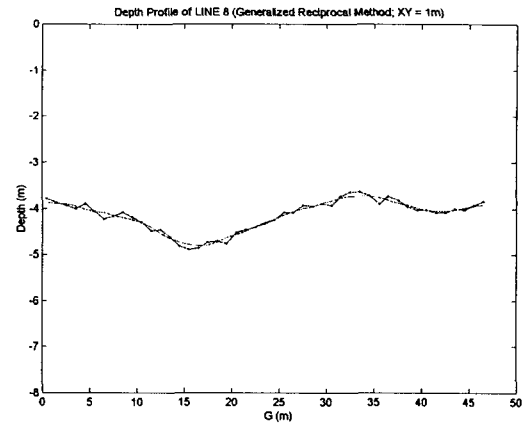
Fig. 7. Depth profile obtained with GRM
