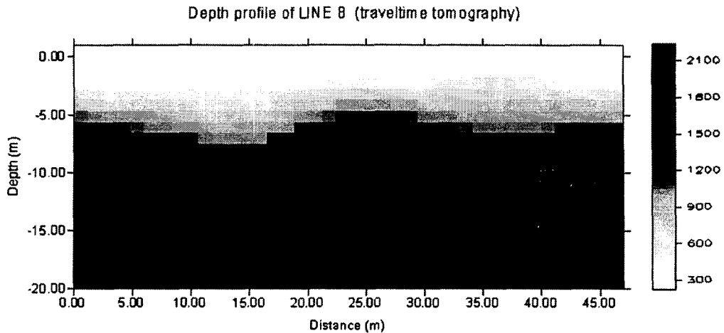
Fig. 8. Depth profile obtained with traveltime tomography.
