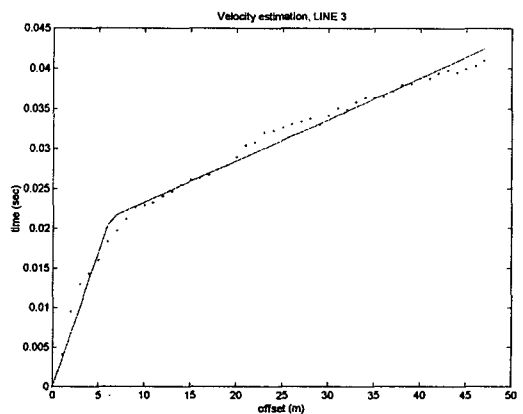
Fig. 2. First arrival fitting
