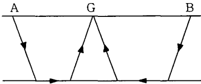
Fig. 3. Reciprocal time method
