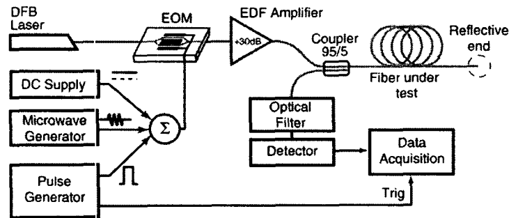
그림 3-2 Experimental set-up for distributed Brillouin gain spectrum measurements.
