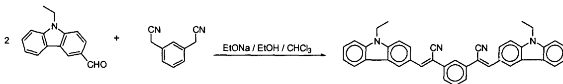
FIGURE 1. Synthesis of BECCIP.
