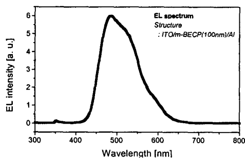
FIGURE 3. EL spectrum of ITO/BECCIP/Al structure.
