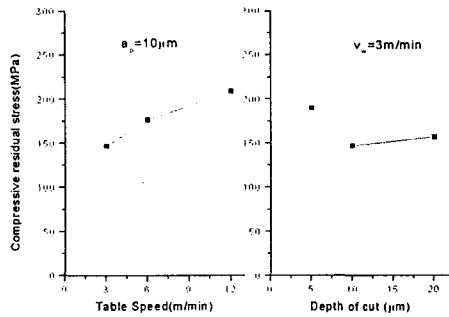
Fig. 10 Grinding conditions versus residual stress for ZrO_2 Ceramic
