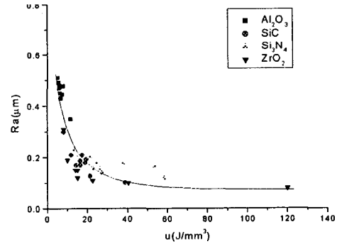
Fig. 8 R_a versus specific grinding energy
