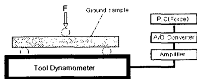
(b) 3 point bending test on machining center
