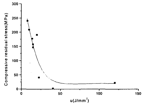
Fig. 12 Specific grinding energy and compressive residual stress
