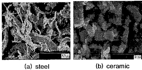
Fig. 2 SEM micrographs of grinding debris of steel and ceramic
