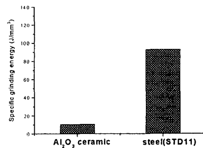
Fig. 5 Specific grinding energy for grinding Al_2O_3 ceramic and tool steel ( a_p = 5 \mu m , v_w = 6 m/min )
