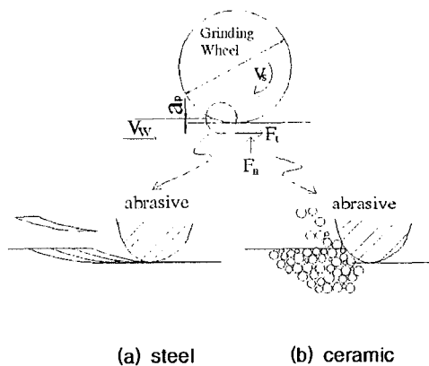
Fig. 4 Grinding mechanisms of steel and ceramic
