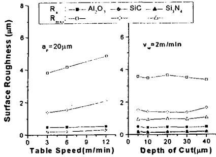
Fig. 6 Grinding conditions versus surface roughness of \text{Al}_2\text{O}_3 , SiC, and \text{Si}_3\text{N}_4
