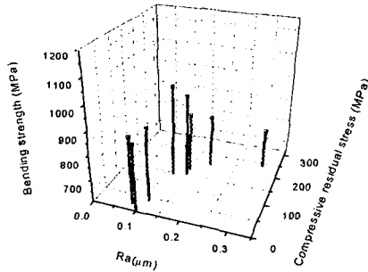
(a) Bending strength, R_a , and residual stress
