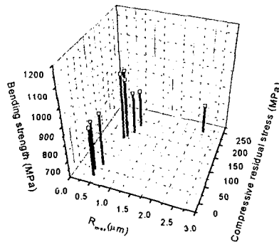
(a) Bending strength, R_{max} , and residual stress Fig. 13 Bending strength of ground ZrO_2 ceramics
