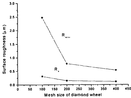
Fig. 7 Mesh size versus surface roughness for grinding of \text{ZrO}_2 ceramic
