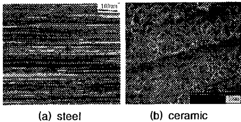
Fig. 3 SEM micrographs of ground surfaces
