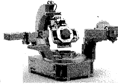
(c) X-ray diffractometer Fig. 1 Experimental system
