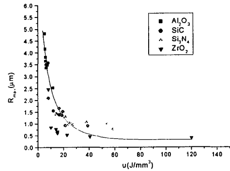
Fig. 9 R_{max} versus specific grinding energy
