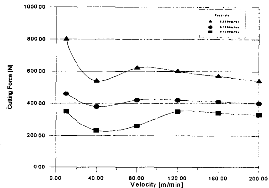
Fig. 1 Experimental Values of Cutting Forces
