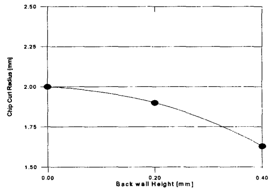
Fig. 6 Effect of Backwall Height on Chip Curl (Groove Width = 2mm)
