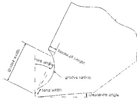
Fig. 4 Nomenclature of Grooved Tool used in FEM Simulations
