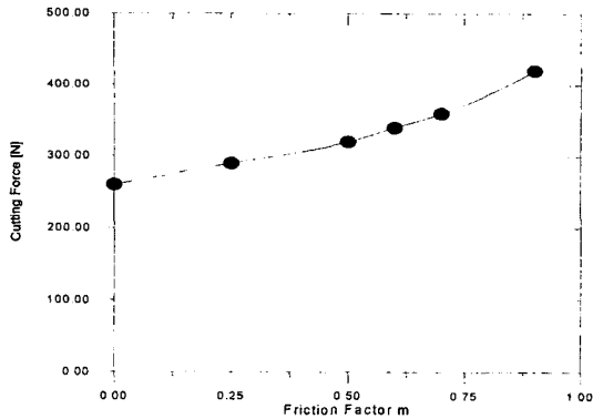
Fig. 2 Variation of Cutting Force with Friction Factor
