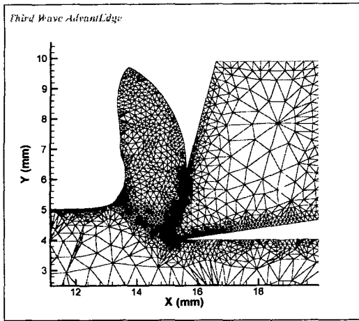
(A) Land less than Depth of Cut
