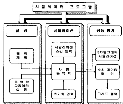
Fig. 2 Structure of Simulator Program
