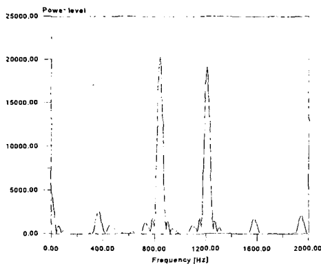
(a) Spectrum of DTMF No.7
