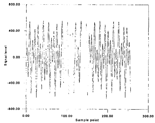
Figure 1 show signals waveform of the DTMF No.1
