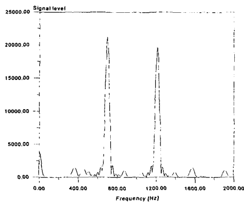
(a) Spectrum of DTMF No. 1
