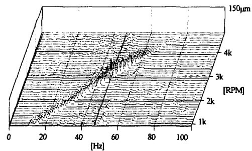
Fig. 7 Variation of the pad fluttering characteristics with the shaft speed (x-axis) ( Q_s=180 //min, W_L=0 kN)
