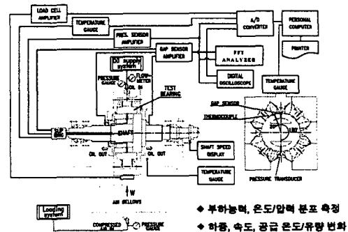
Fig. 2 Schematic diagram of test apparatus
