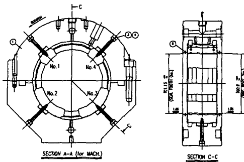
Fig. 3 Test bearing
