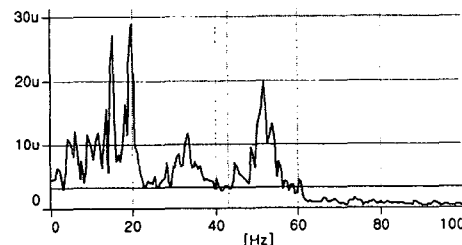
Fig. 5(b) Spectrum of gap sensor (x-axis) ( N=3600 rpm, Q_s=90 //min, W_L=0 kN)
