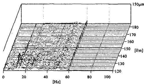
Fig. 8 Variation of the pad fluttering characteristics with the oil supply flow rate (x-axis) ( N=3600 rpm, W_L=0 kN)
