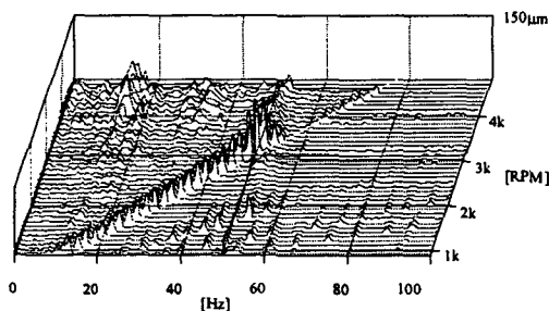
Fig. 6 Variation of the pad fluttering characteristics with the shaft speed (x-axis) ( Q_s=120 //min, W_L=0 kN)
