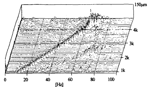
Fig. 9(b) Variation of the pad fluttering characteristics (x-axis) ( W_L=10 kN, Q_s=120 //min)
