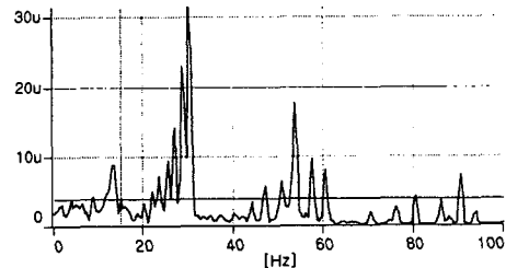
Fig. 5(a) Spectrum of gap sensor (x-axis) ( N=1800 rpm, Q_s=90 //min, W_L=0 kN)
