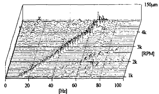
Fig. 9(a) Variation of the pad fluttering characteristics (x-axis) ( W_L=5 kN, Q_s=120 //min)
