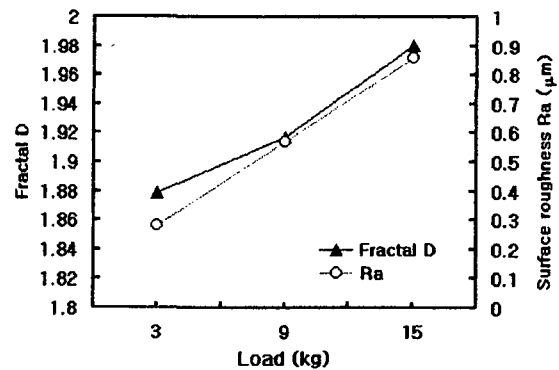
Fig. 5 A comparison between surface roughness and fractal dimension
