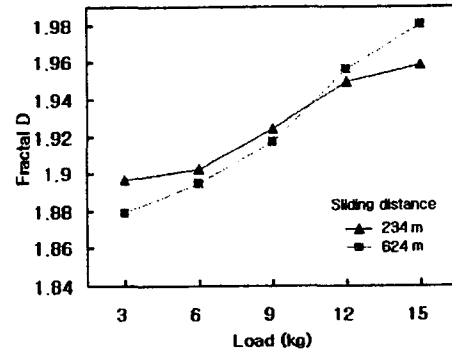
Fig. 7 Effect of applied load on fractal dimension
