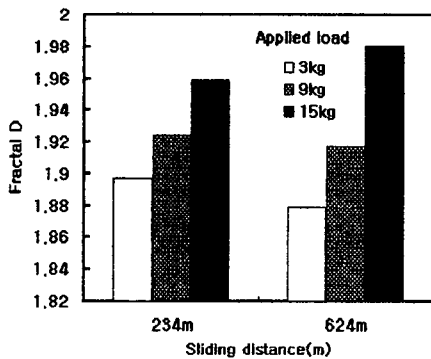
Fig. 10 Fractal dimension vs sliding distance and applied load
