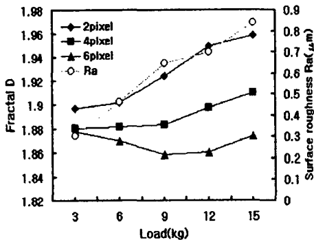
Fig. 6 Effect of step size on fractal dimension
