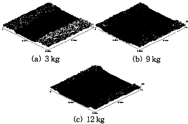
Fig. 9 3D model of rubbed surface on applied load, sliding distance : 234 m
