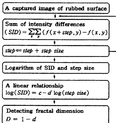
Fig. 4 Flow chart of algorithm for fractal dimension
