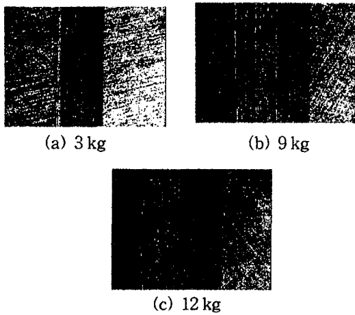
Fig. 8 Image of rubbed surface on applied load, sliding distance : 234 m
