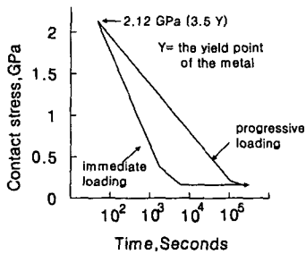
Fig. 1. The durability of steel sliding surfaces with lubricants comparing systems where full loads were applied immediately and progressively [2].
