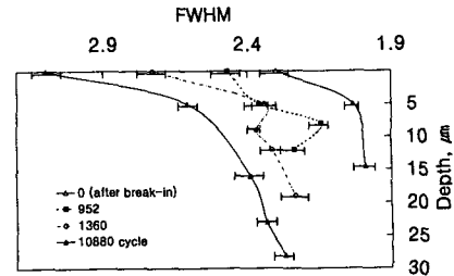
Fig. 7. The degree of plastic deformation during the scuffing test with break-in
