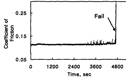
(b) With break-in
