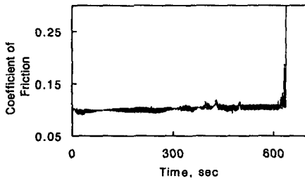
(a) Without break-in
