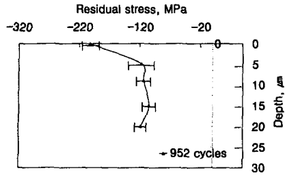
(c) After 952 cycles
