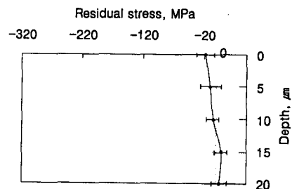
(a) Before the scuffing test
