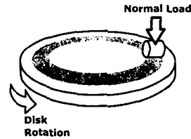
Fig. 2. Cylinder-on-disk type sliding test
