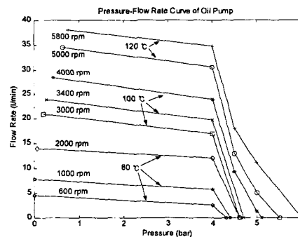
Fig. 2 The Flow Characteristics of Oil Pump
