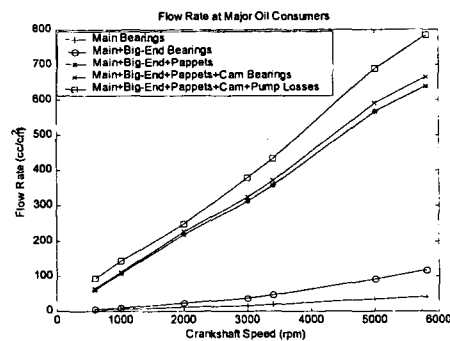
Fig. 12 Flow Rate vs. RPM at Main Oil Consumer
