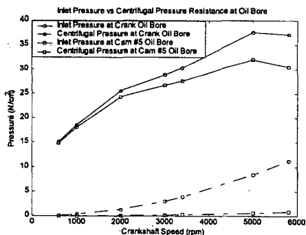
Fig. 13 Bearing Entrance Pressure vs. Centrifugal Pressure at Big-End Bearing and Cam Bearing
