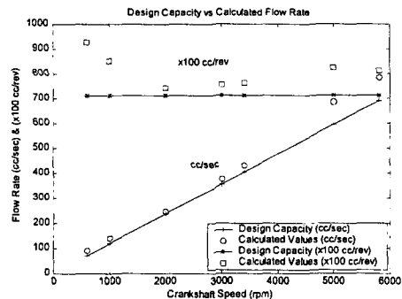
Fig. 8 Theoretical vs. Calculated Flow Rate
