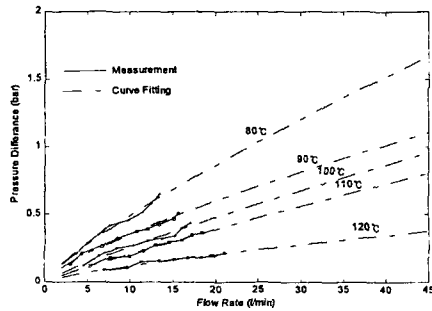
Fig. 3 The Flow Characteristics of Oil Filter
