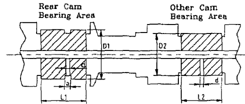
Fig. 4 The Schematic Drawing of Camshaft around Bearing Area
