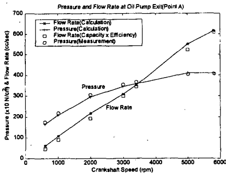
Fig. 9 Pressure and Flow Rate at Oil Pump Exit The measuring data of pressure at point A, B and C in Fig. 1 are compared to the calculated values at each RPM in Fig. 10.
