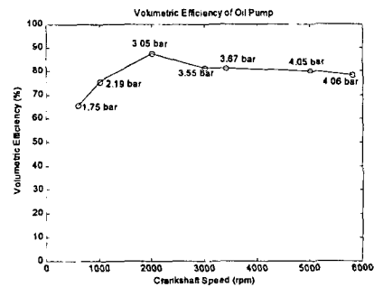
Fig. 7 Volumetric Efficiency of Oil Pump
