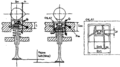
Fig. 5 The Geometry of Hydraulic Tappet and The Flow Schematic Drawing
