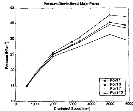
Fig. 11 Pressure vs. RPM at Main Calculated Points
