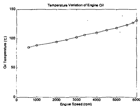
Fig. 6 Temperature of Engine Oil
