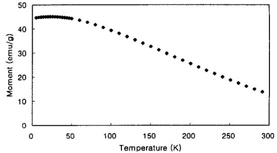
Fig. 2. Temperature dependence of magnetization of the ultrafine Zn-ferrite particles
