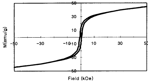
Fig. 1. Magnetic hysteresis loop of the ultrafine Zn-ferrite particles at 5K.
