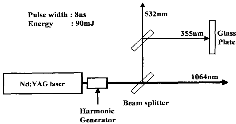
Figure. 1. Schematic of Nd:YAG laser emitting Third Harmonic Generated 355nm wavelength with repetition of 10Hz and 8ns pulse duration.
