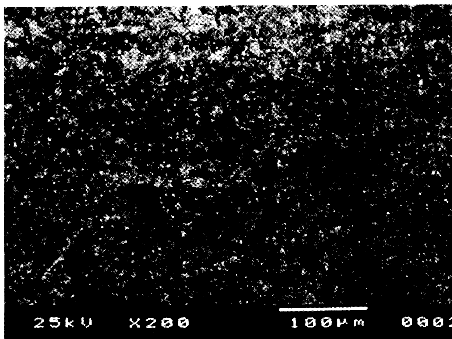
Figure. 4. SEM photograph of \text{LiAlSi}_3\text{O}_8 phases in the photosensitive glass after laser irradiation of 355nm wavelength and heat treatment at 570°C for 1h. The acid leaching by diluted HF was carried out.
