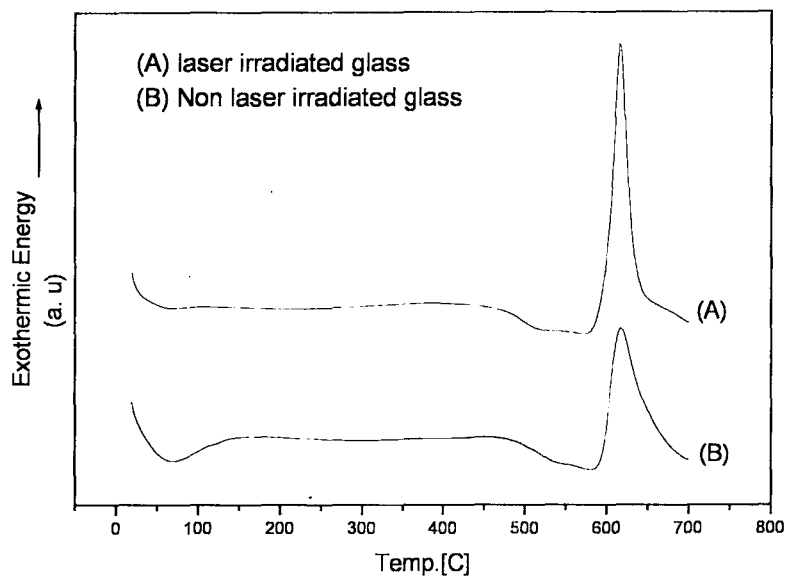
Figure. 2. Differential Thermal Calorimetry traces of laser irradiated glass(A) and non-laser irradiated glass(B). The exothermic peaks are indicating crystallization in each glass.
