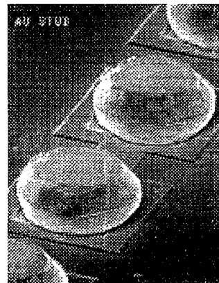
Figure 1 (a). Scanning electron microscopy of coined Au stud bumps formed on Al pads of test chip.
