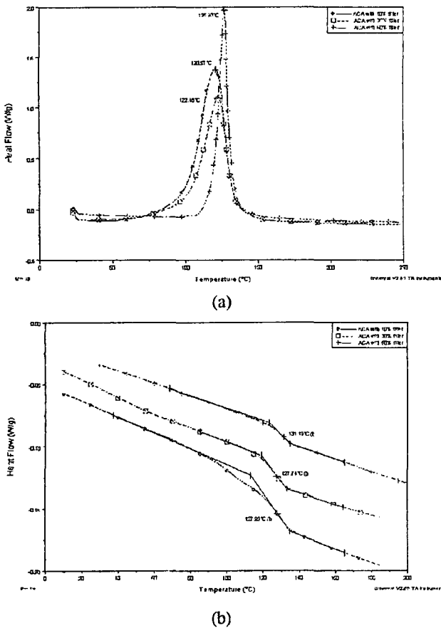
Figure 3. DSC curves of ACA samples with nickel and silica fillers of different contents (10, 30, 50 wt.%) Effect of the filler contents on (a) the curing profiles and (b) the glass transition curves of three ACA composites.
