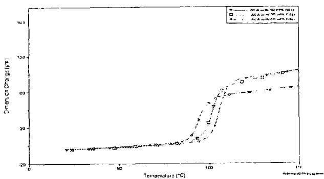
Figure 5. TMA curves of three ACA composite samples with different content of fillers.
