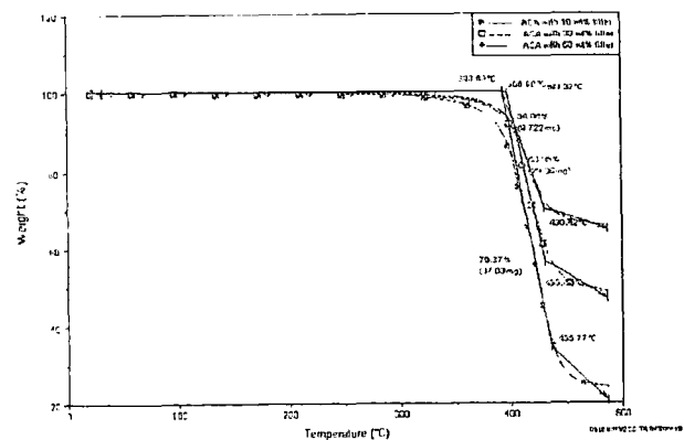
Figure 6. TGA curves of three ACA samples with different content fillers
