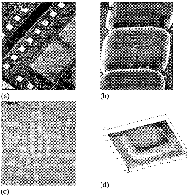
Fig. 1 (b) Electroless Ni Bumps (a) unbumped Si chip, (b) Ni bumps, (c) surface morphology, and (d) configuration of Ni/Au bump.
