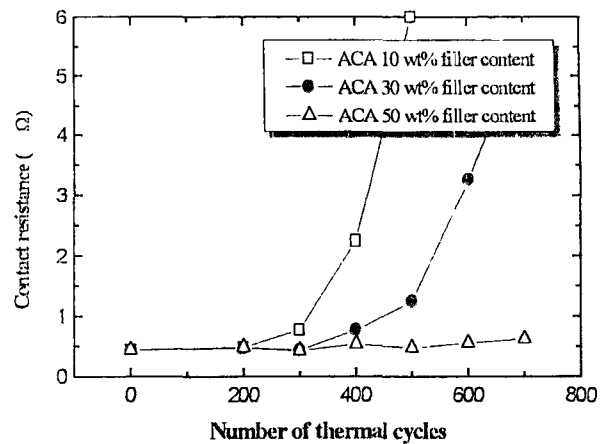
Figure 8. Contact resistance of flip chip interconnects using ACA with different filler content during thermal cycling test from -60^{\circ}\text{C} to 150^{\circ}\text{C} for 700 cycles
