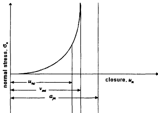
Fig. 2. Parameters used to calculate normal stress during loading cycle.
