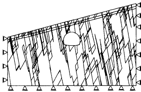
Fig. 7. Model and boundary conditions.
