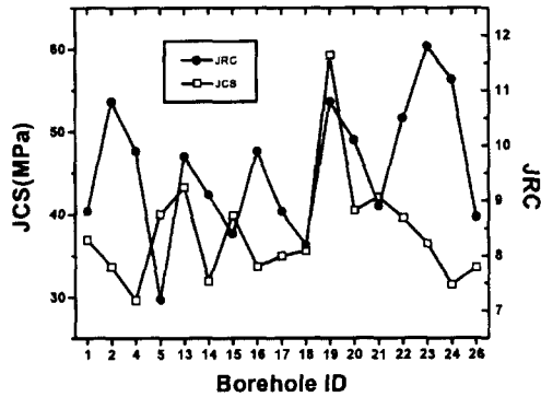
Fig. 5. Variations of JRC and JCS in boreholes.
