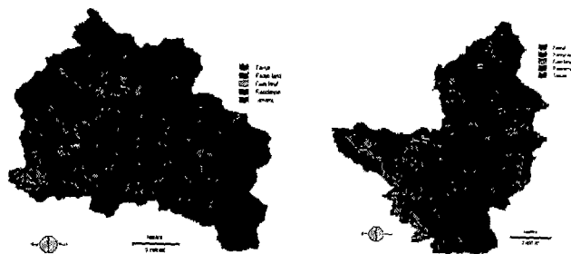
Fig. 4. Landuse map of Study area
