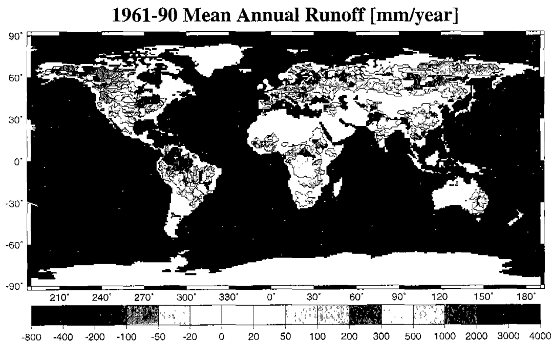
Figure 3: Mean annual runoff (mm/y) based on gauge data mean 1961-90.
