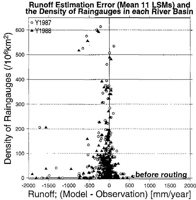
Figure 5: Comparisons between the density of raingauges [ /10^6\text{km}^2 ] used in preparing the forcing precipitation and the mean bias error [mm/y] of 11 LSMs.
