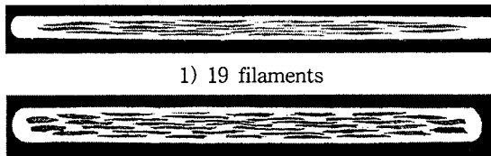
Fig.1 Cross-section of Bi-2223/Ag HTS tapes
