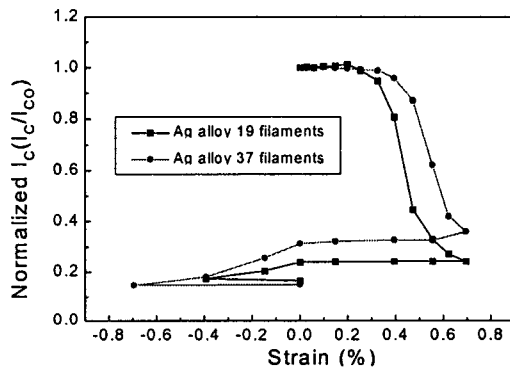
Fig.4 The effect of number of filaments in the strain- I_c measurement
