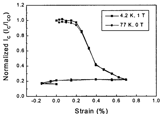
Fig.5 The normalized critical current versus axial strain strains, measured at different temperature (77, 4.2 K) and magnetic field( B=0, 1 T).
