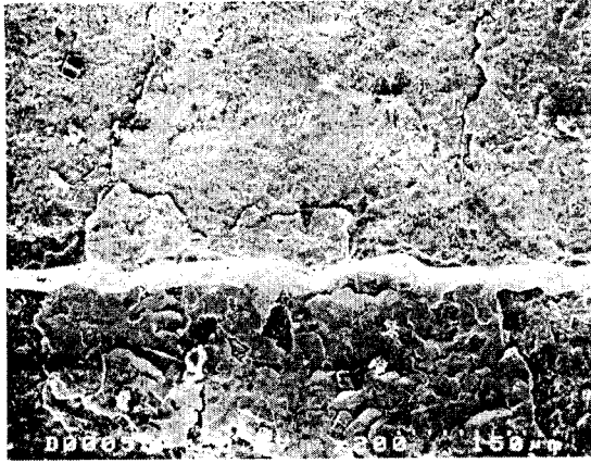
Fig.6 Fracture propagation between the superconducting filaments.
