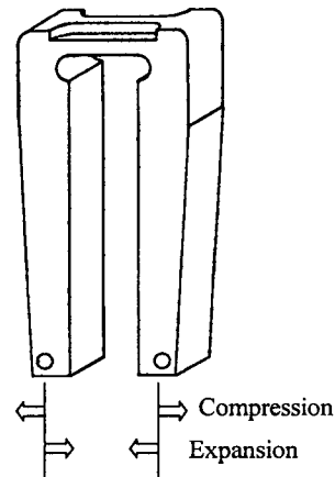
Fig.2 U-shape sample holder for Bi-2223/Ag HTS tapes
