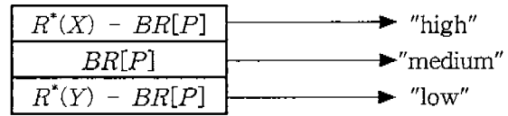
Fig. 2. approximation space partition for quantitative attribute values
