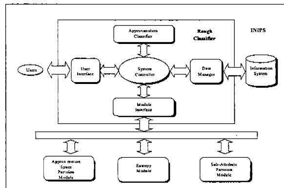
Fig. 3. Structure of INiPS
