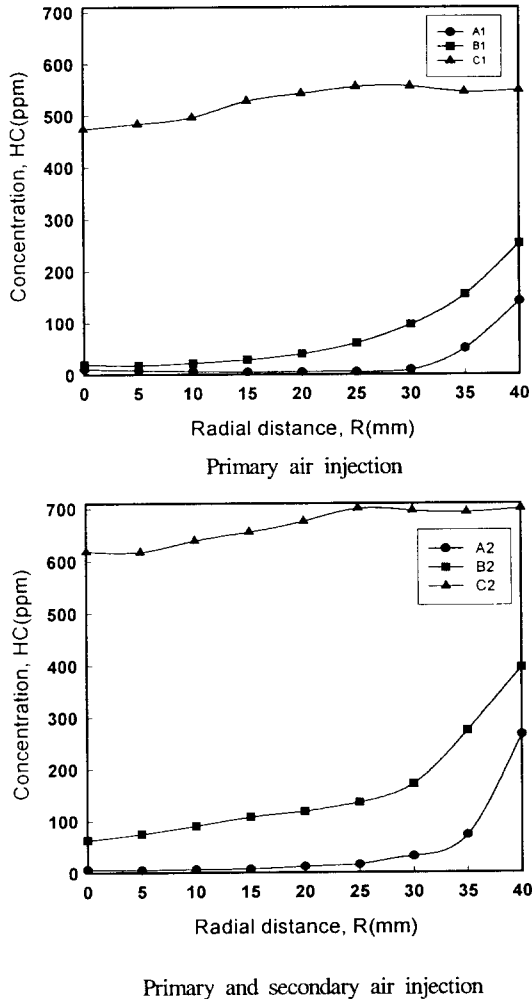
Fig. 9 Distributions of HC concentration for A1, B1, C1 and A2, B2, C3 at Z=200mm
