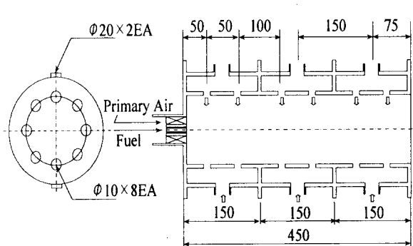
Fig. 2 Detail of model gas turbine combustor
