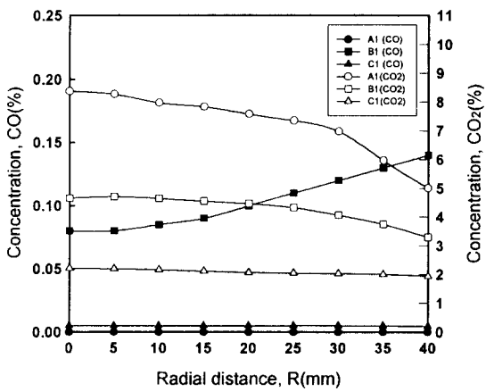
Fig. 7 Distributions of CO, CO 2 concentration for A1, B1, C1
