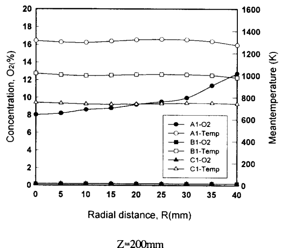
Fig. 5 Distributions of O_2 , meantemperature for A1, B1, C1
