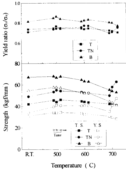
Fig. 7 Effect of degradation temperature and time on the tensile properties of specimens
