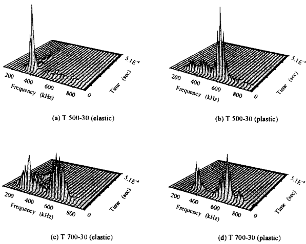
Fig. 10 Time-frequency analysis for elastic and plastic area of T specimen
