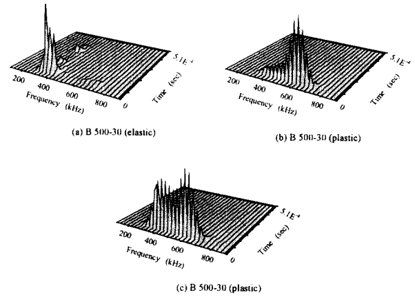
Fig. 11 Time-frequency analysis for elastic and plastic area of B specimen
