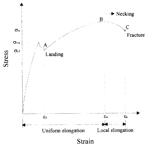
Fig. 4 Typical nominal stress - strain curve
