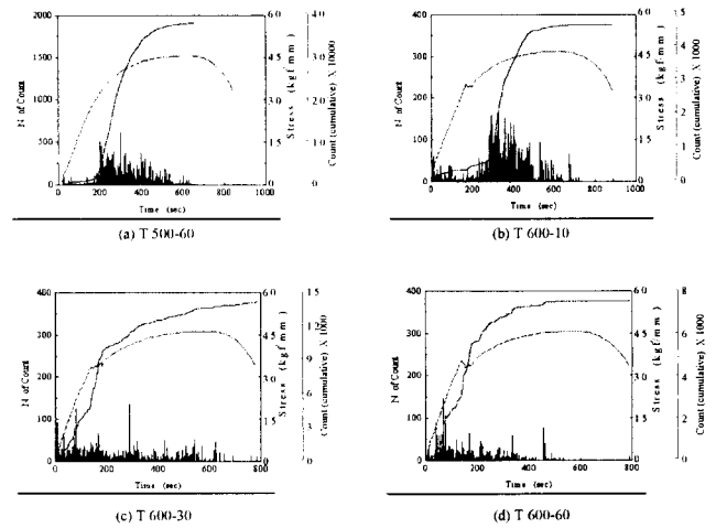
Fig. 8 AE count produced during the tensile test of T specimen
