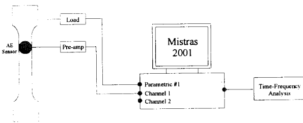
Fig. 3 Schematic diagram of AE system
