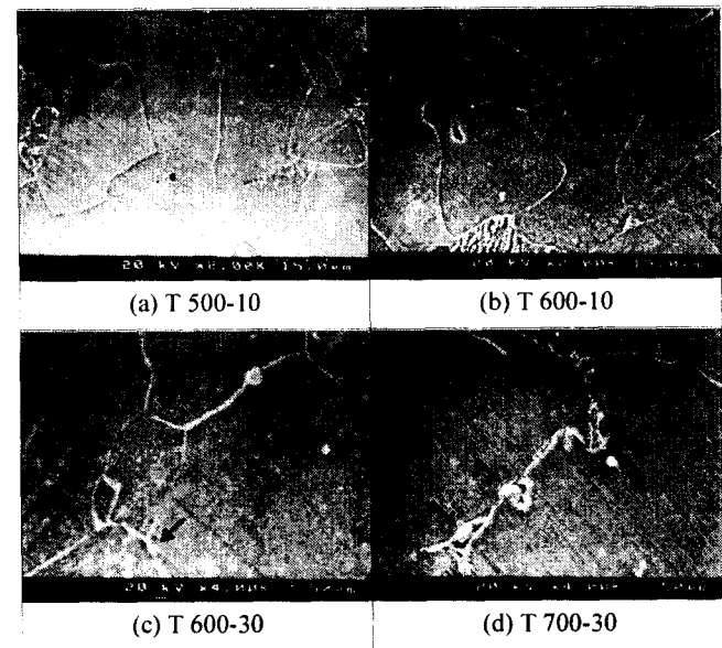
Fig. 6 SEM micrographs showing the T specimen
