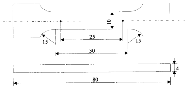
Fig. 2 Dimension of tensile specimen (in mm)
