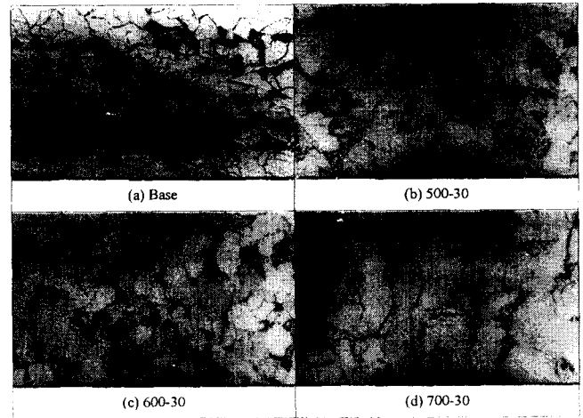
Fig. 5 Optical micrographs showing the T specimen by degradation temperature
