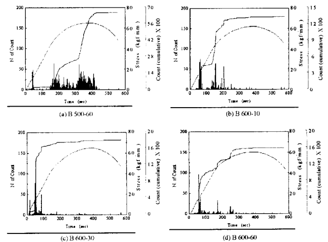
Fig. 9 AE count produced during the tensile test of B specimen
