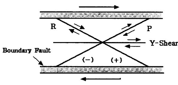
Fig. 1. Secondary shears developed in gouge layers.
