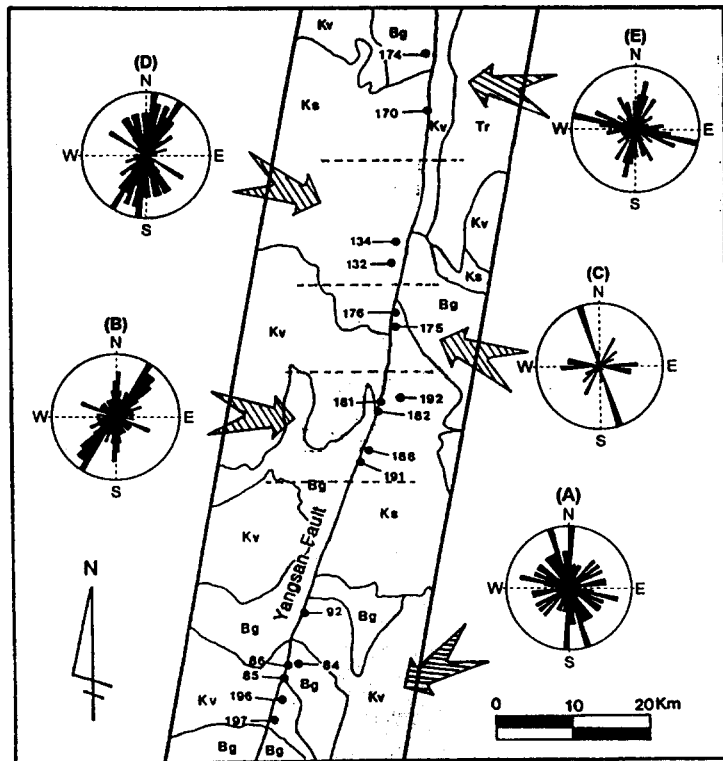
Fig. 3. Geological map and outcrop localities of small faults measured. KS : Hayang Group; Kv:Yucheon Group; Bg: Bulguksa Granite; Tr:Tertiary rocks. Dashed lines are the domain boundaries.
