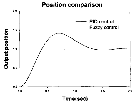
Fig. 2 Output position trend comparison
