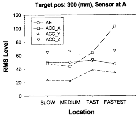
Fig. 8 RMS level at A (target position 300 mm)
