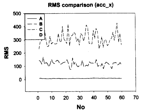
Fig. 6 Acc_x level
