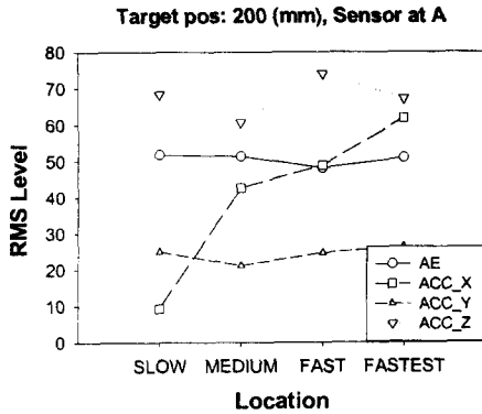
Fig. 7 RMS level at A (target position 200 mm)
