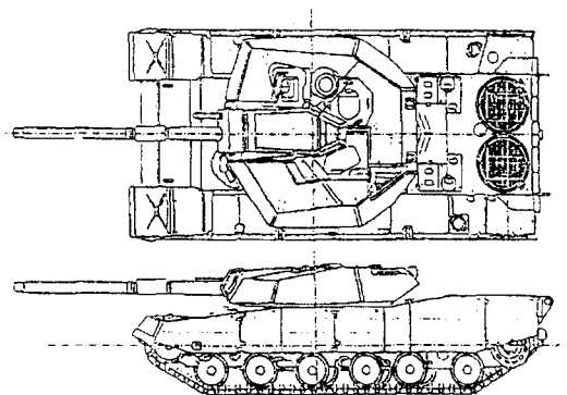
Fig.1 External of Track Vehicle
