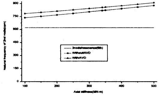
Fig. 6 Natural frequency of 2nd Node axial vibration for 9K80MC-S engine
