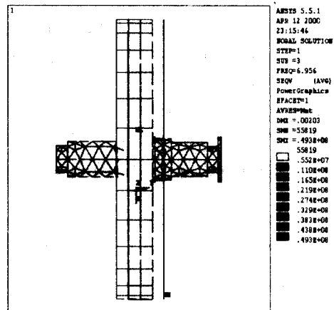
Fig. 3 Natural frequency and mode shape of generator rotor rim (0,0 mode)
