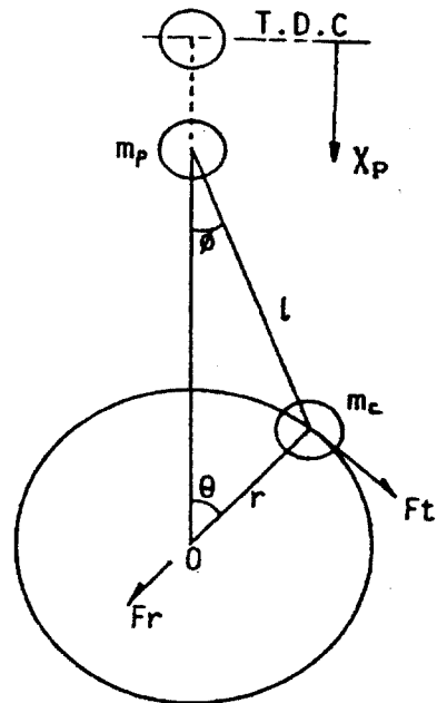
Fig. 2 Inertia force of crank and piston
