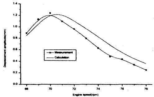
Fig. 14 The 6th order disp. amp. of crankshaft free end with AVD inactive
