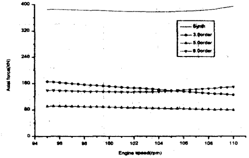
Fig. 9 Axial force between gen. shaft and rotor rim with full load and AVD active condition
