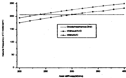
Fig. 5 Natural frequency of 0 node axial vibration for 9K80MC-S engine
