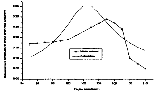
Fig. 13 The 2nd order displacement amp. of crankshaft free end with AVD inactive
