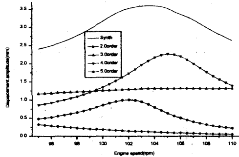
Fig. 10 The displacement amp. of crank shaft free end with AVD inactive and full load
