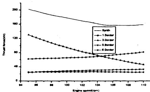
Fig. 8 Thrust force of thrust bearing with full load and AVD active condition
