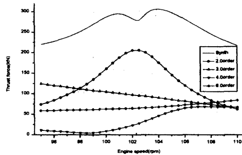
Fig. 11 The thrust force of thrust bearing with AVD inactive and full load
