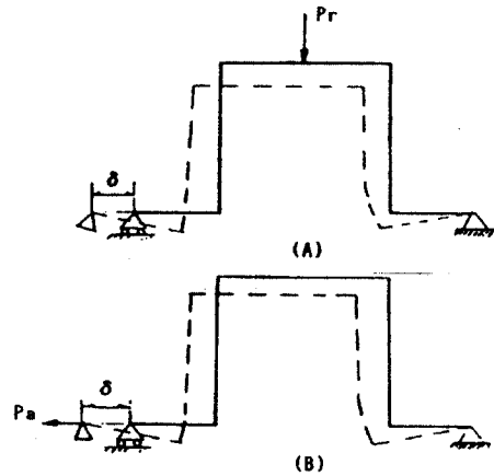
Fig. 1 Conversion of the radial force to the axial force
