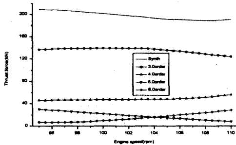
Fig. 7 Thrust force of axial damper with full load and AVD active condition
