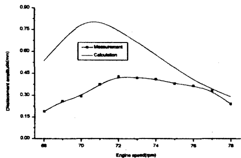
Fig. 15 The 6th order displacement amp. of rotor rim end with AVD inactive
