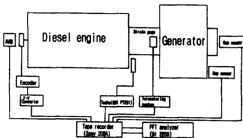
Fig.12 Schematic diagram for axial-torsional coupled vibration measurement
