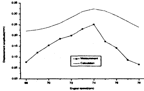
Fig. 16 The 6th order displacement amp. of crankshaft free end with AVD active
