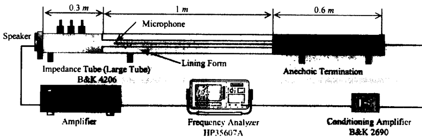
Figure 1. Experimental setup
